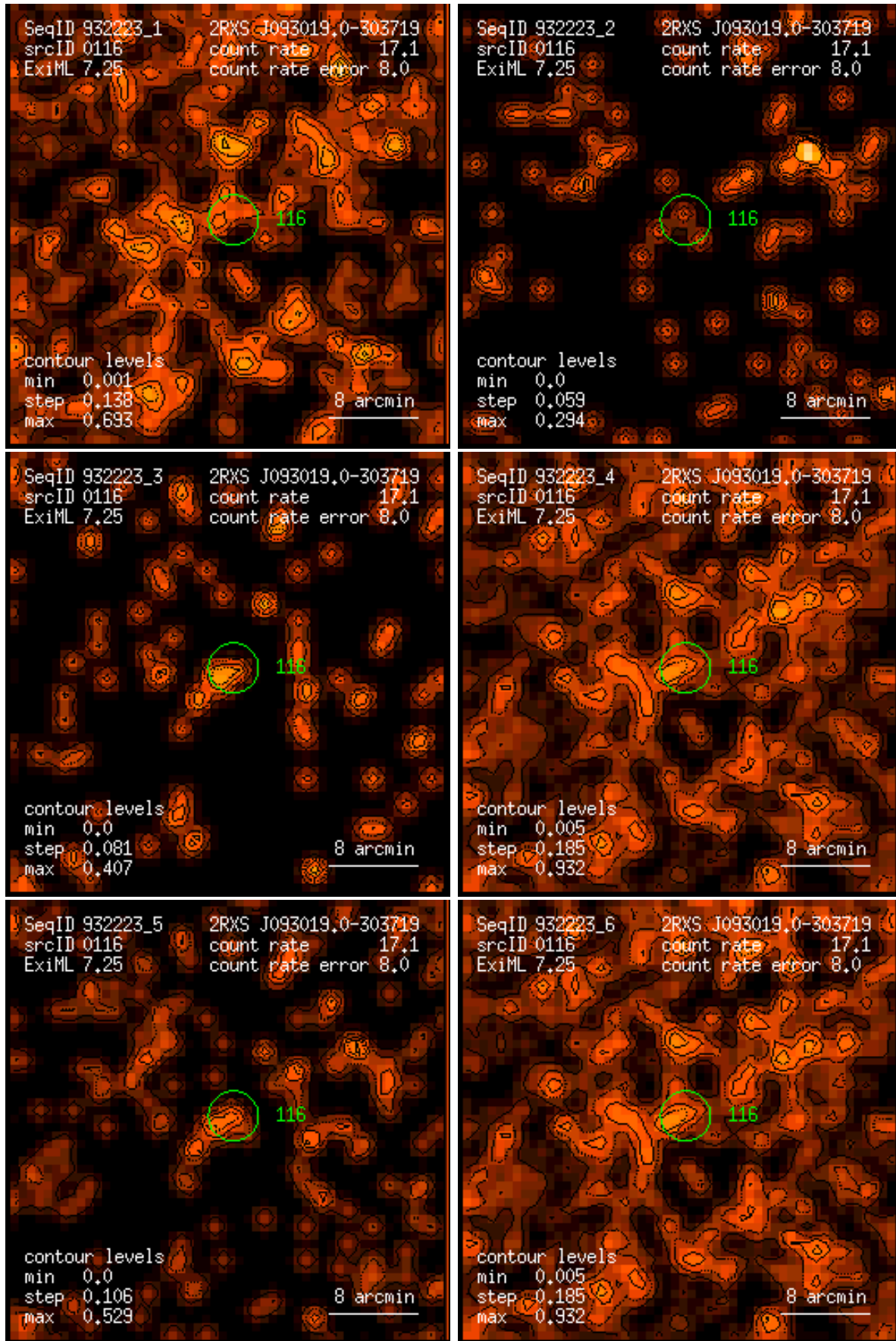
Figure 116: RASS 932223: detection 0116: band rate images, Gaussian filter: (1) PSPC channels 11 – 41, (2) 52 – 90, (3) 91 – 201, (4) 11 – 235, (5) 52 – 201, (6) 11 – 201. Broad band rates in counts/ks. Band rate contour levels in counts/ks/arcmin 2 .
