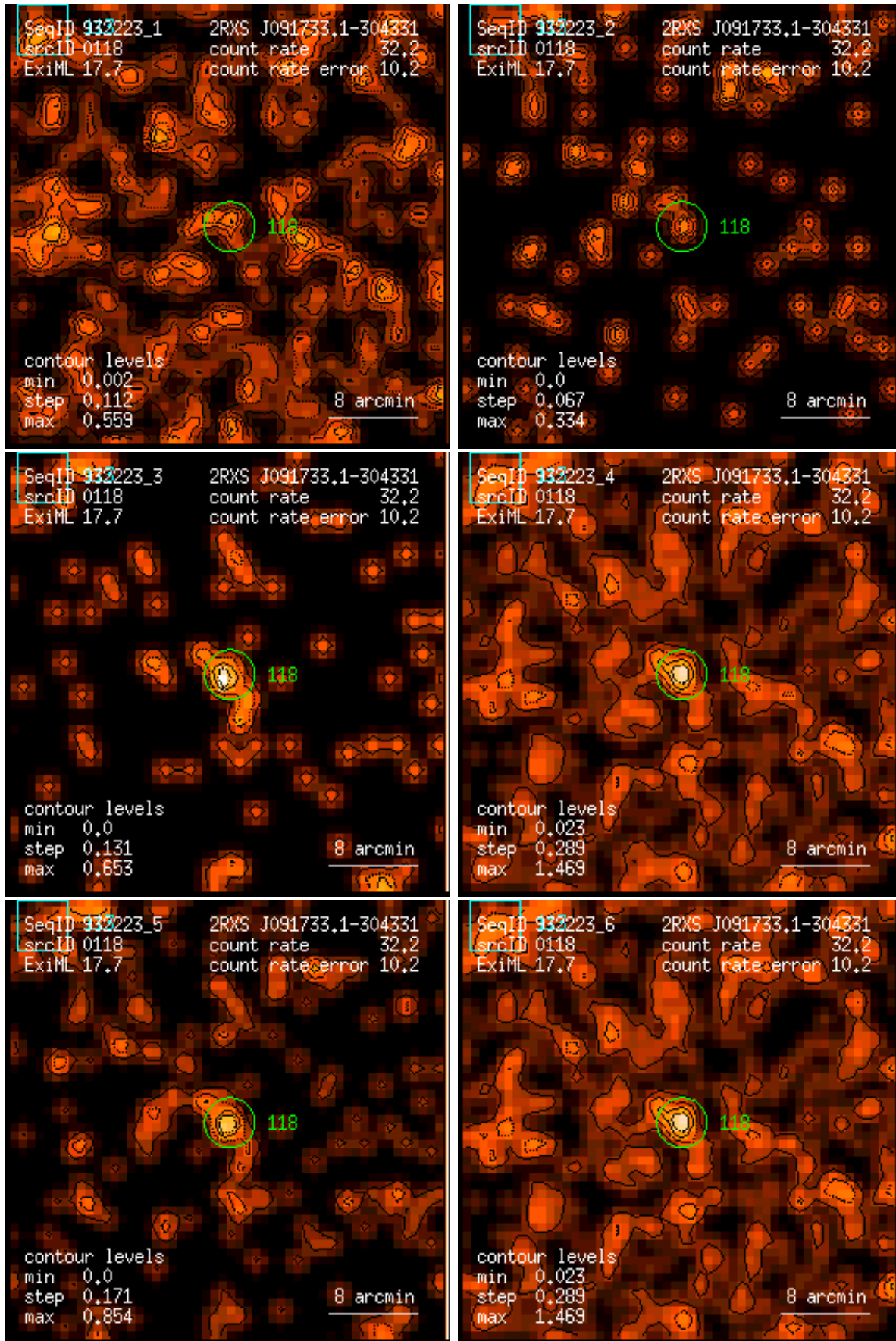
Figure 118: RASS 932223: detection 0118: band rate images, Gaussian filter: (1) PSPC channels 11 – 41, (2) 52 – 90, (3) 91 – 201, (4) 11 – 235, (5) 52 – 201, (6) 11 – 201. Broad band rates in counts/ks. Band rate contour levels in counts/ks/arcmin 2 .
