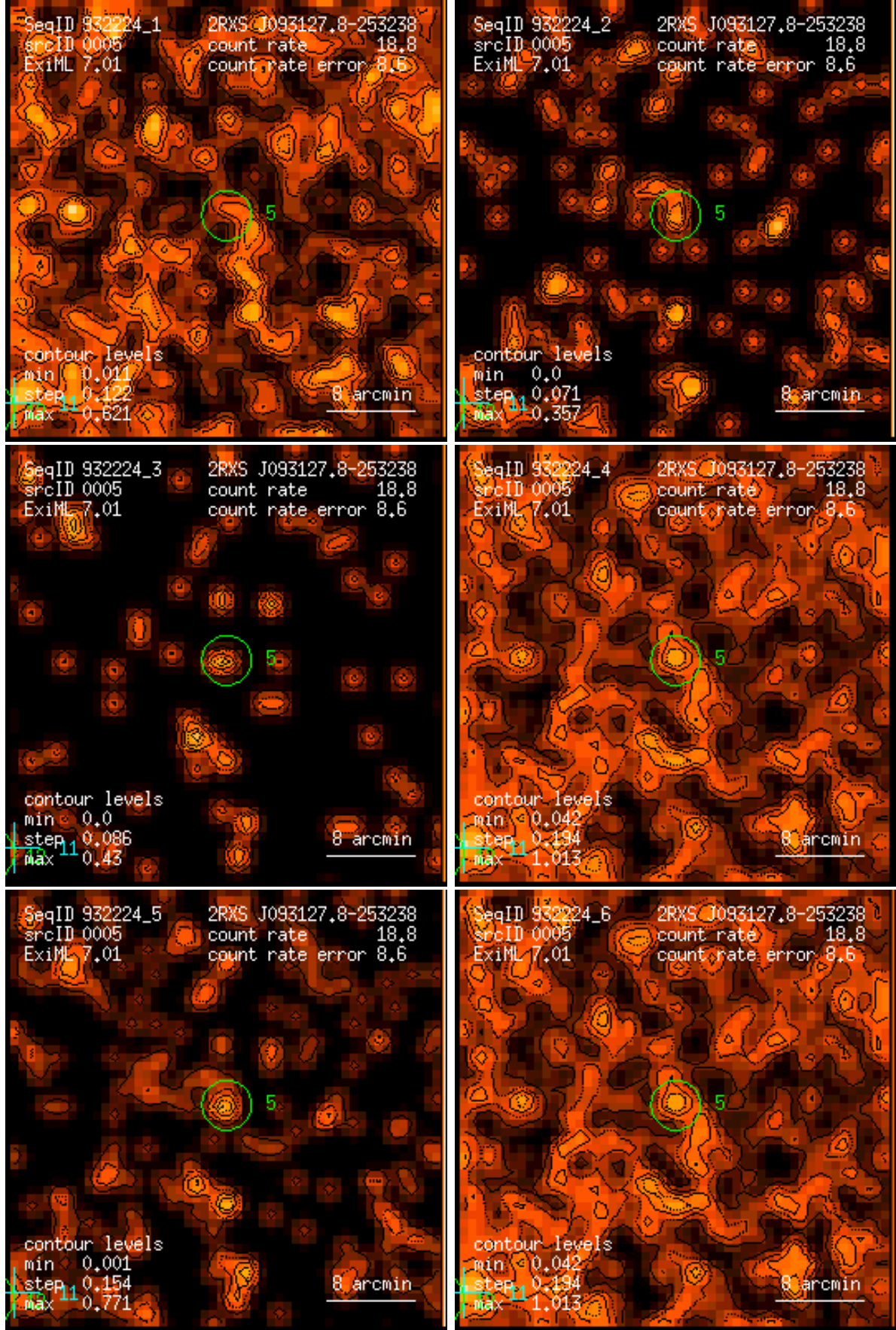
Figure 5: RASS 932224: detection 0005: band rate images, Gaussian filter: (1) PSPC channels 11 – 41, (2) 52 – 90, (3) 91 – 201, (4) 11 – 235, (5) 52 – 201, (6) 11 – 201. Broad band rates in counts/ks. Band rate contour levels in counts/ks/arcmin 2 .
