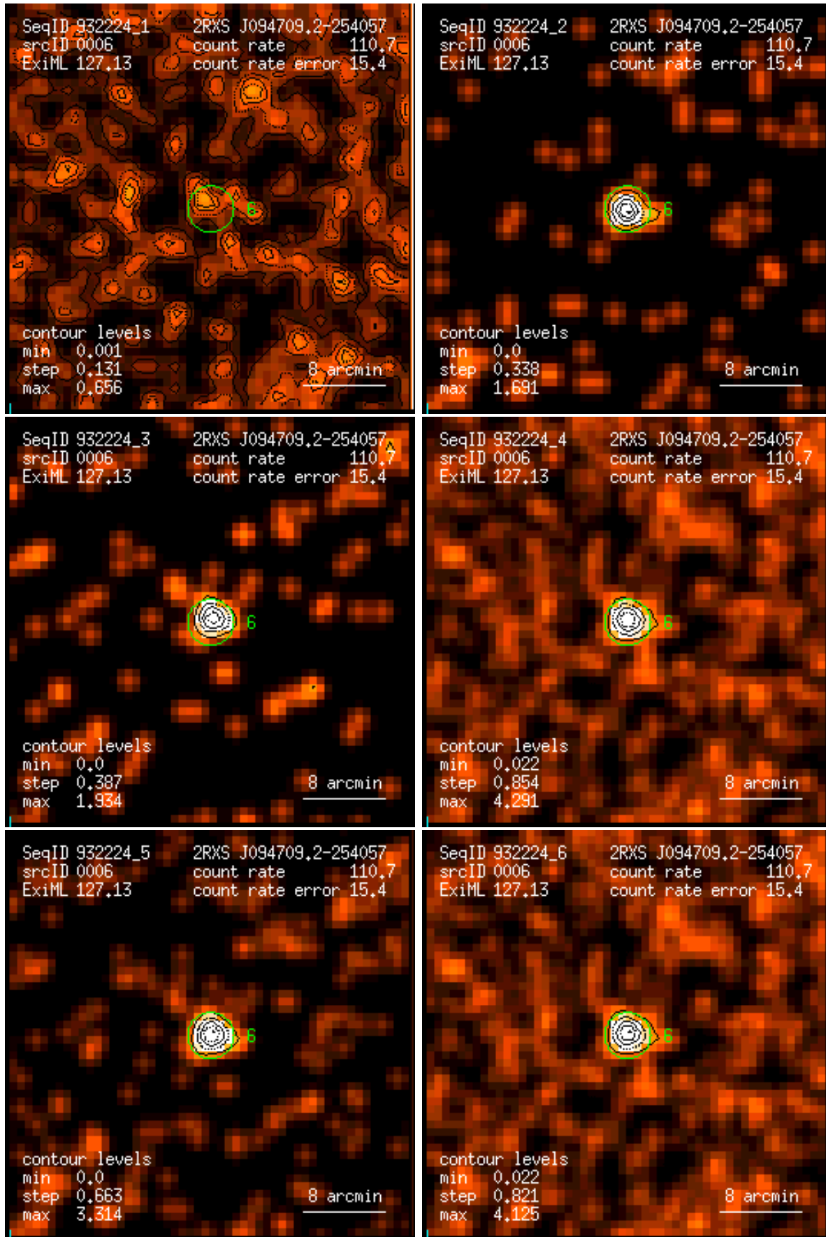
Figure 6: RASS 932224: detection 0006: band rate images, Gaussian filter: (1) PSPC channels 11 – 41, (2) 52 – 90, (3) 91 – 201, (4) 11 – 235, (5) 52 – 201, (6) 11 – 201. Broad band rates in counts/ks. Band rate contour levels in counts/ks/arcmin 2 .
