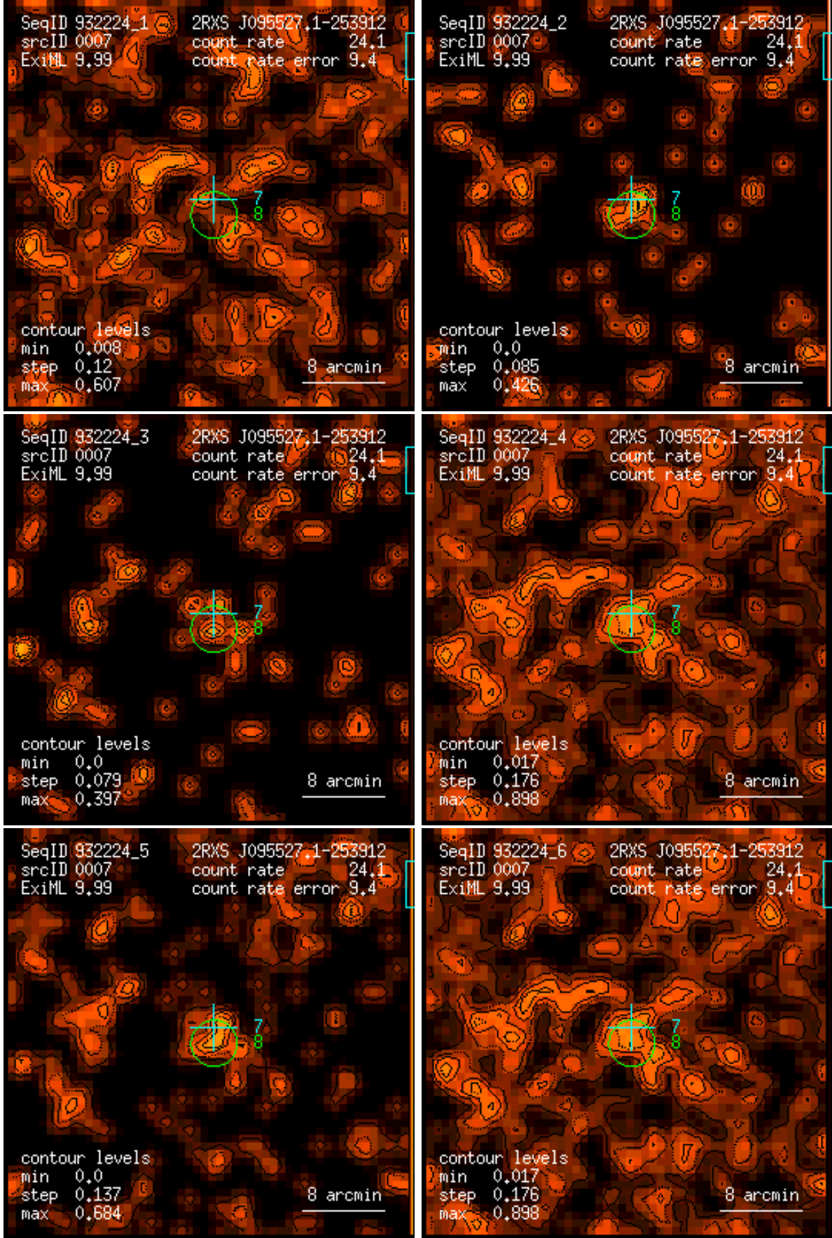
Figure 7: RASS 932224: detection 0007: band rate images, Gaussian filter: (1) PSPC channels 11 – 41, (2) 52 – 90, (3) 91 – 201, (4) 11 – 235, (5) 52 – 201, (6) 11 – 201. Broad band rates in counts/ks. Band rate contour levels in counts/ks/arcmin 2 .
