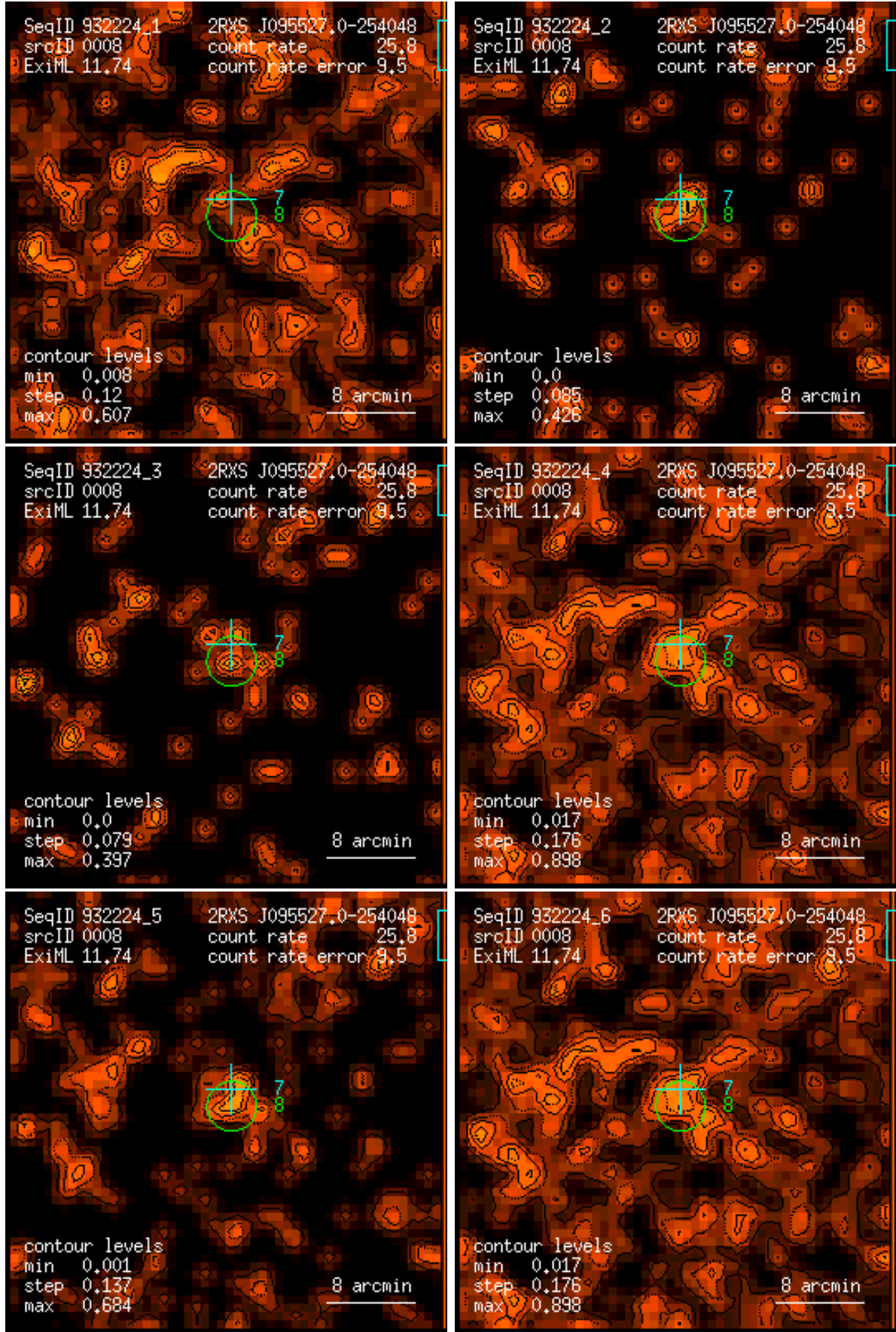
Figure 8: RASS 932224: detection 0008: band rate images, Gaussian filter: (1) PSPC channels 11 – 41, (2) 52 – 90, (3) 91 – 201, (4) 11 – 235, (5) 52 – 201, (6) 11 – 201. Broad band rates in counts/ks. Band rate contour levels in counts/ks/arcmin 2 .
