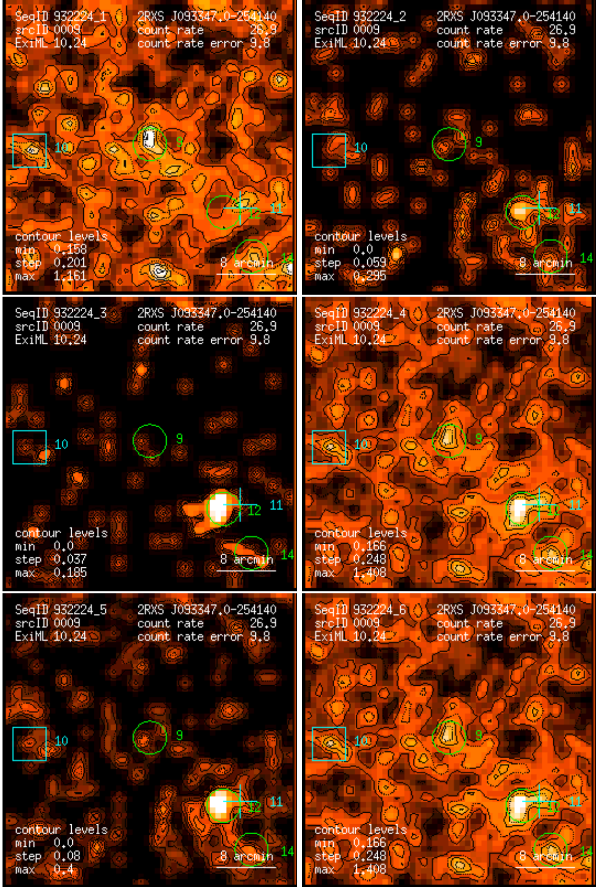
Figure 9: RASS 932224: detection 0009: band rate images, Gaussian filter: (1) PSPC channels 11 – 41, (2) 52 – 90, (3) 91 – 201, (4) 11 – 235, (5) 52 – 201, (6) 11 – 201. Broad band rates in counts/ks. Band rate contour levels in counts/ks/arcmin 2 .
