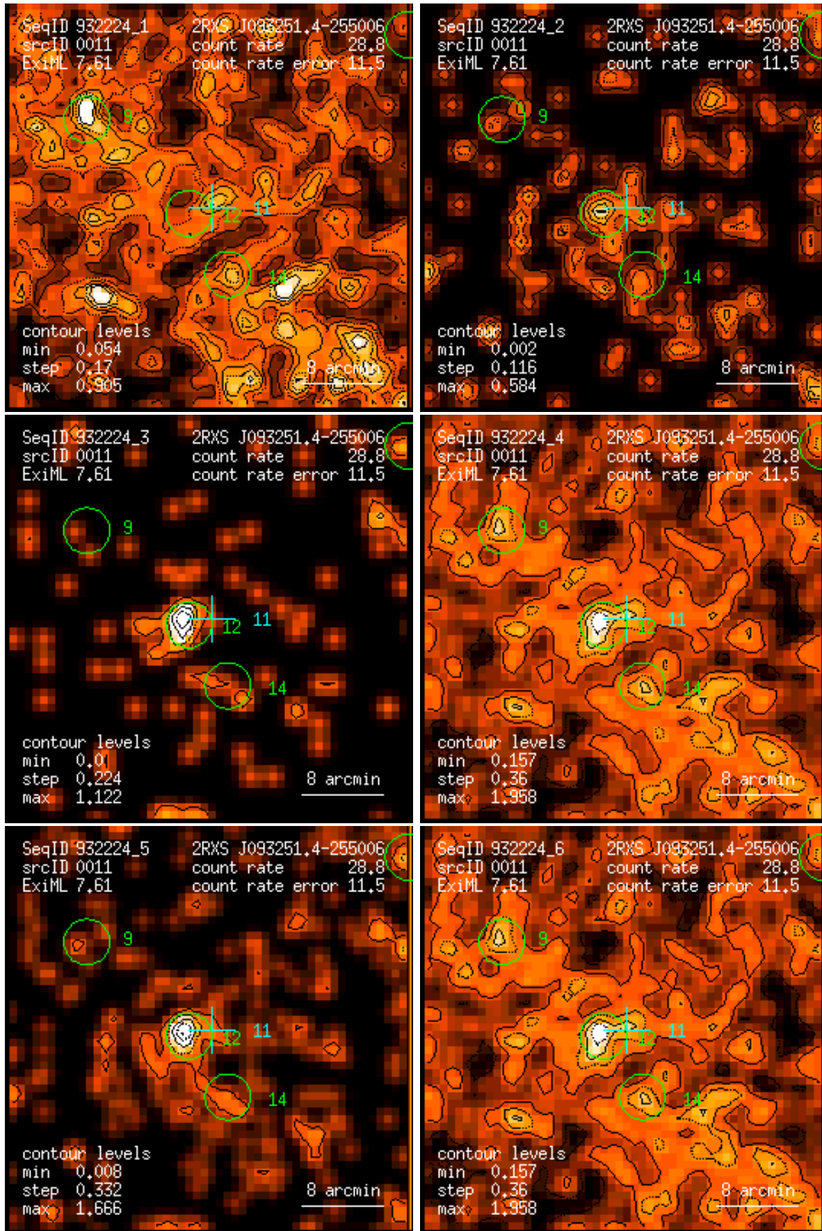
Figure 11: RASS 932224: detection 0011: band rate images, Gaussian filter: (1) PSPC channels 11 – 41, (2) 52 – 90, (3) 91 – 201, (4) 11 – 235, (5) 52 – 201, (6) 11 – 201. Broad band rates in counts/ks. Band rate contour levels in counts/ks/arcmin 2 .
