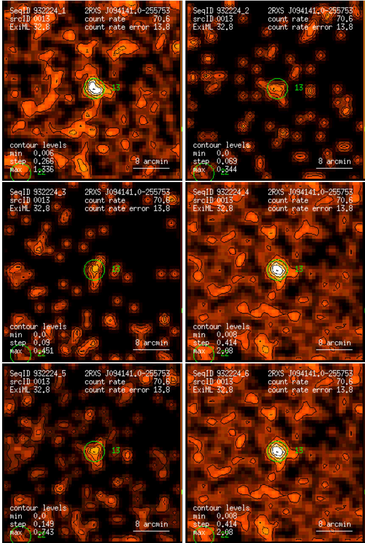
Figure 13: RASS 932224: detection 0013: band rate images, Gaussian filter: (1) PSPC channels 11 – 41, (2) 52 – 90, (3) 91 – 201, (4) 11 – 235, (5) 52 – 201, (6) 11 – 201. Broad band rates in counts/ks. Band rate contour levels in counts/ks/arcmin 2 .
