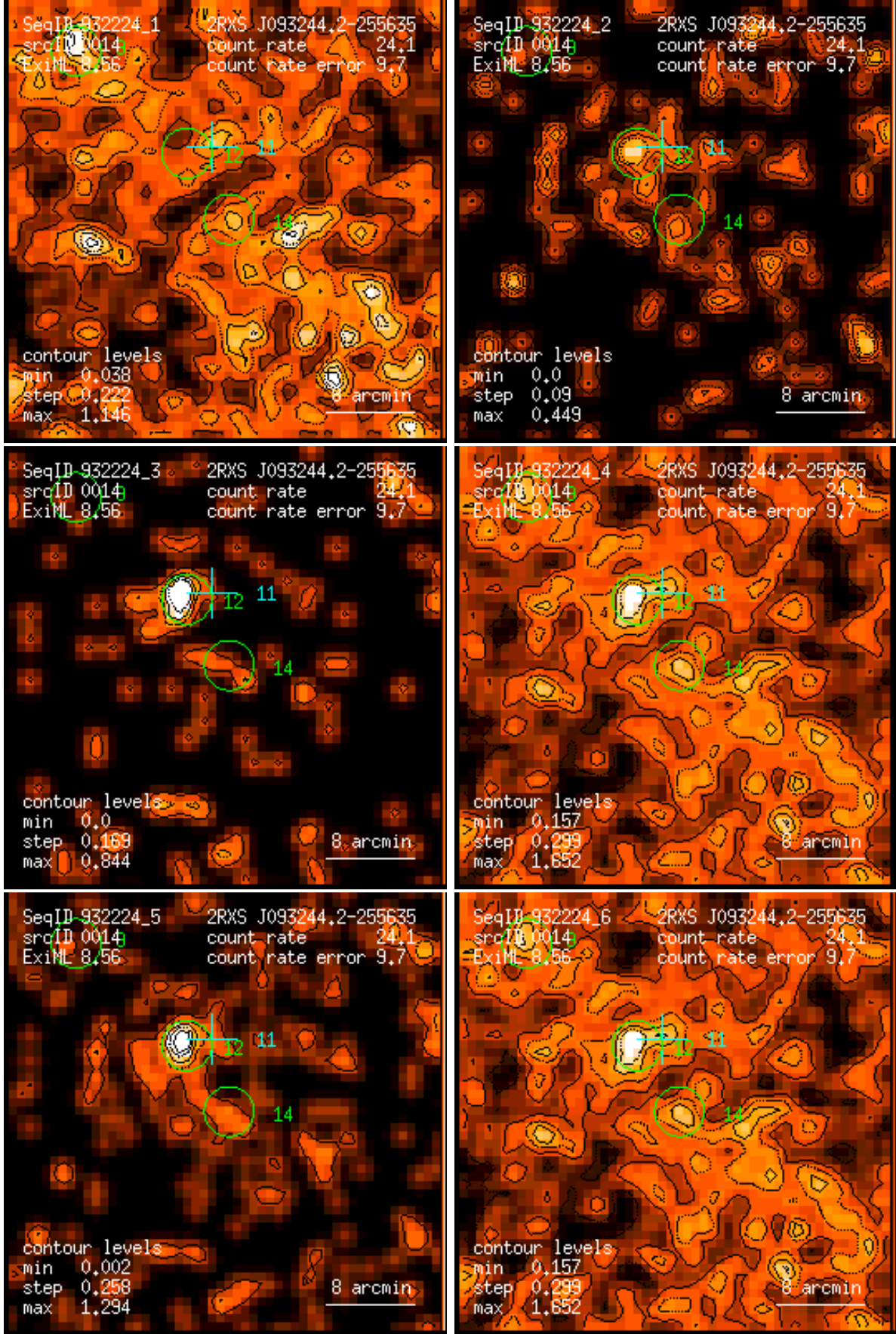
Figure 14: RASS 932224: detection 0014: band rate images, Gaussian filter: (1) PSPC channels 11 – 41, (2) 52 – 90, (3) 91 – 201, (4) 11 – 235, (5) 52 – 201, (6) 11 – 201. Broad band rates in counts/ks. Band rate contour levels in counts/ks/arcmin 2 .
