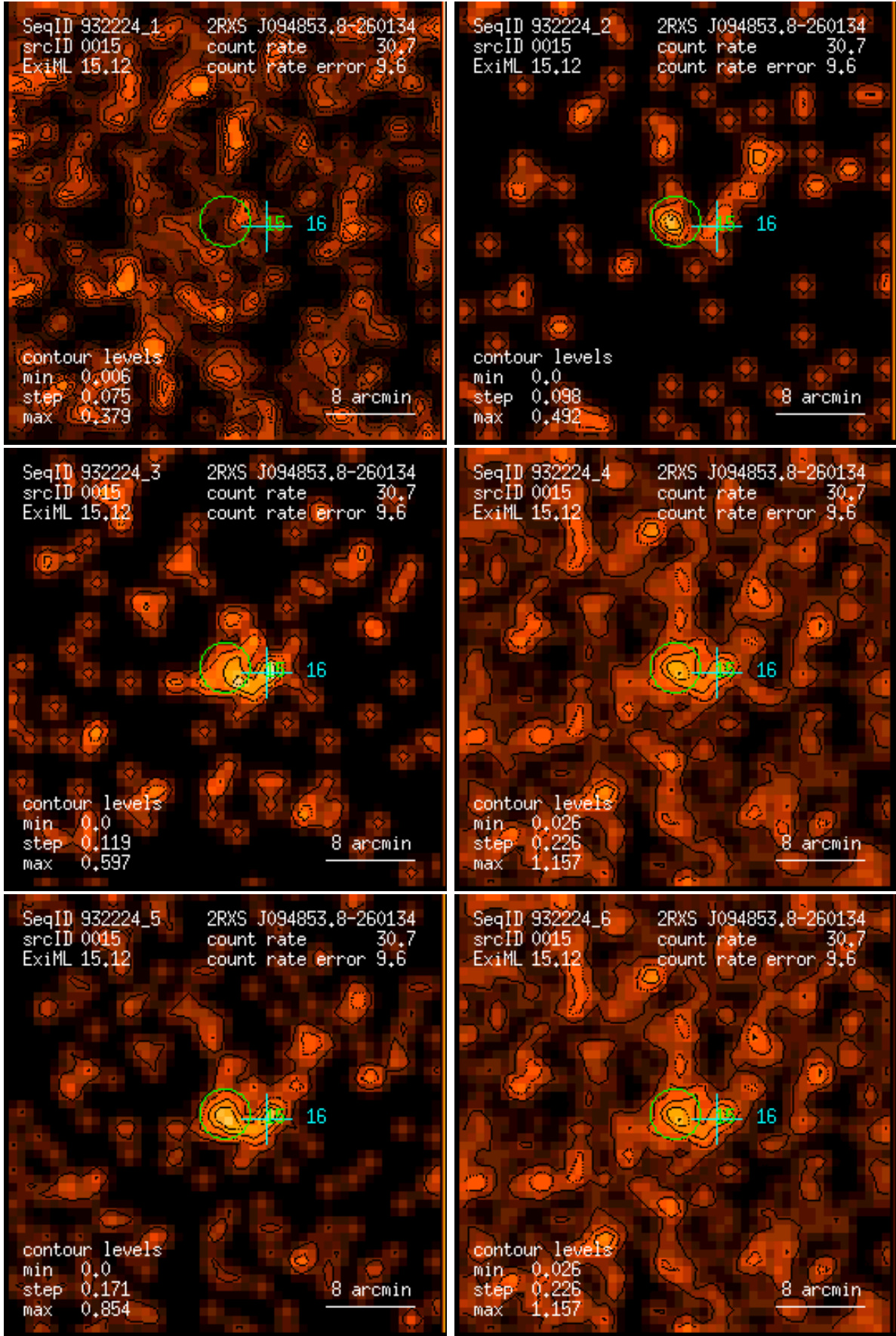
Figure 15: RASS 932224: detection 0015: band rate images, Gaussian filter: (1) PSPC channels 11 – 41, (2) 52 – 90, (3) 91 – 201, (4) 11 – 235, (5) 52 – 201, (6) 11 – 201. Broad band rates in counts/ks. Band rate contour levels in counts/ks/arcmin 2 .
