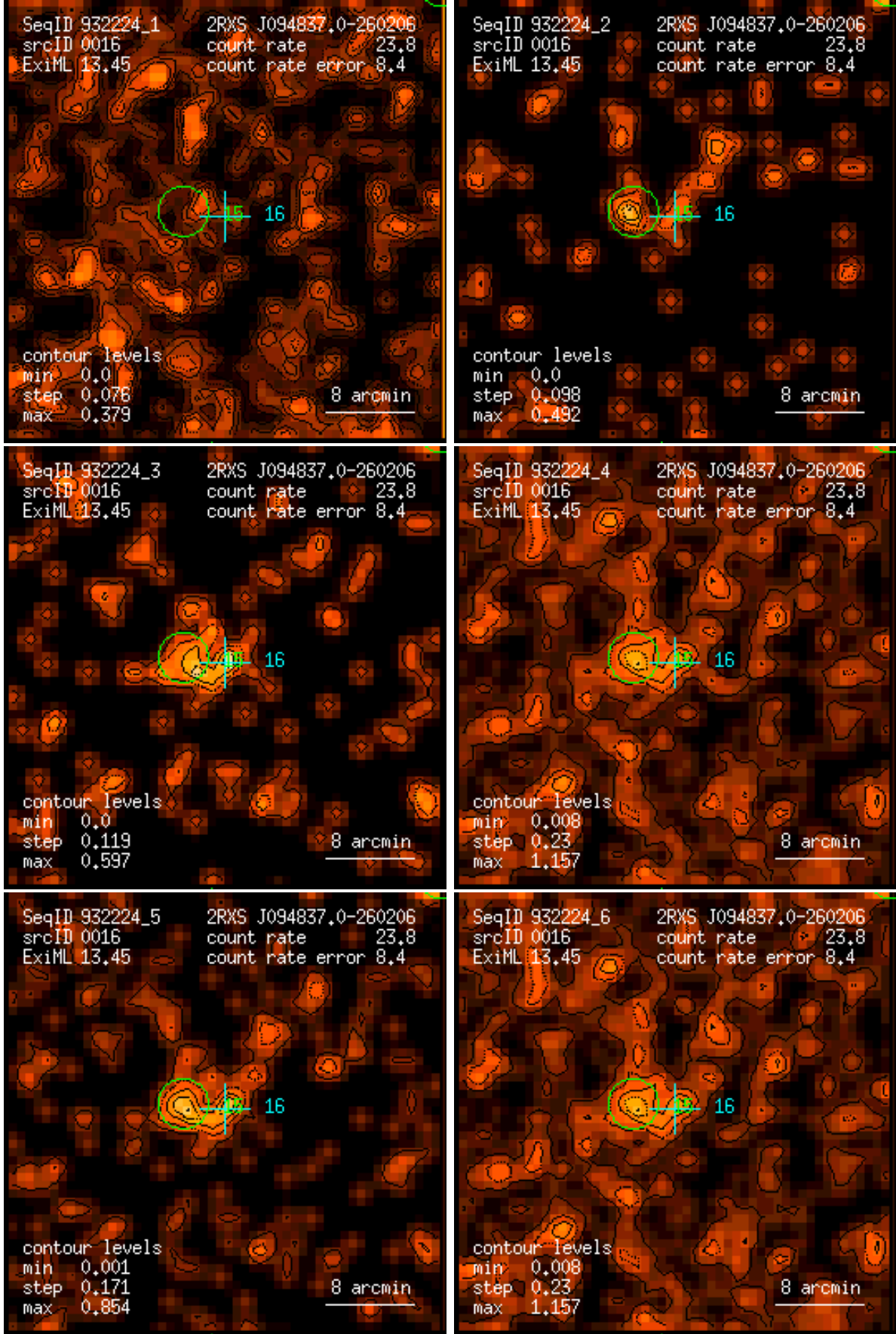
Figure 16: RASS 932224: detection 0016: band rate images, Gaussian filter: (1) PSPC channels 11 – 41, (2) 52 – 90, (3) 91 – 201, (4) 11 – 235, (5) 52 – 201, (6) 11 – 201. Broad band rates in counts/ks. Band rate contour levels in counts/ks/arcmin 2 .
