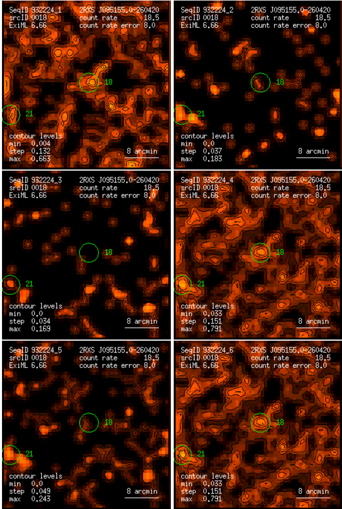
Figure 18: RASS 932224: detection 0018: band rate images, Gaussian filter: (1) PSPC channels 11 – 41, (2) 52 – 90, (3) 91 – 201, (4) 11 – 235, (5) 52 – 201, (6) 11 – 201. Broad band rates in counts/ks. Band rate contour levels in counts/ks/arcmin 2 .
