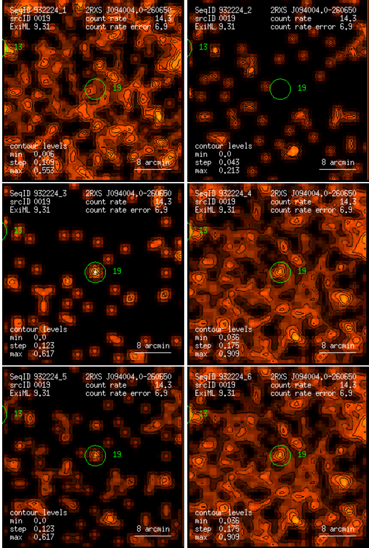
Figure 19: RASS 932224: detection 0019: band rate images, Gaussian filter: (1) PSPC channels 11 – 41, (2) 52 – 90, (3) 91 – 201, (4) 11 – 235, (5) 52 – 201, (6) 11 – 201. Broad band rates in counts/ks. Band rate contour levels in counts/ks/arcmin 2 .
