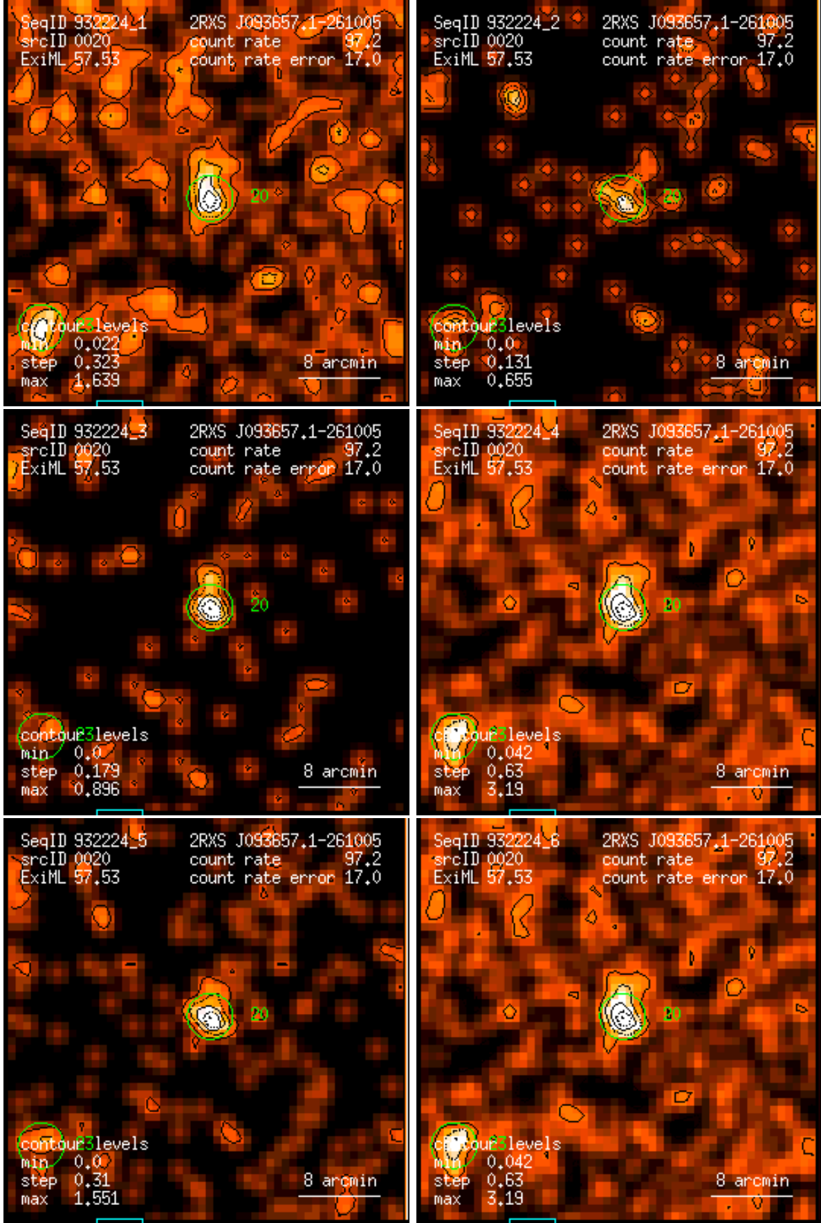
Figure 20: RASS 932224: detection 0020: band rate images, Gaussian filter: (1) PSPC channels 11 – 41, (2) 52 – 90, (3) 91 – 201, (4) 11 – 235, (5) 52 – 201, (6) 11 – 201. Broad band rates in counts/ks. Band rate contour levels in counts/ks/arcmin 2 .
