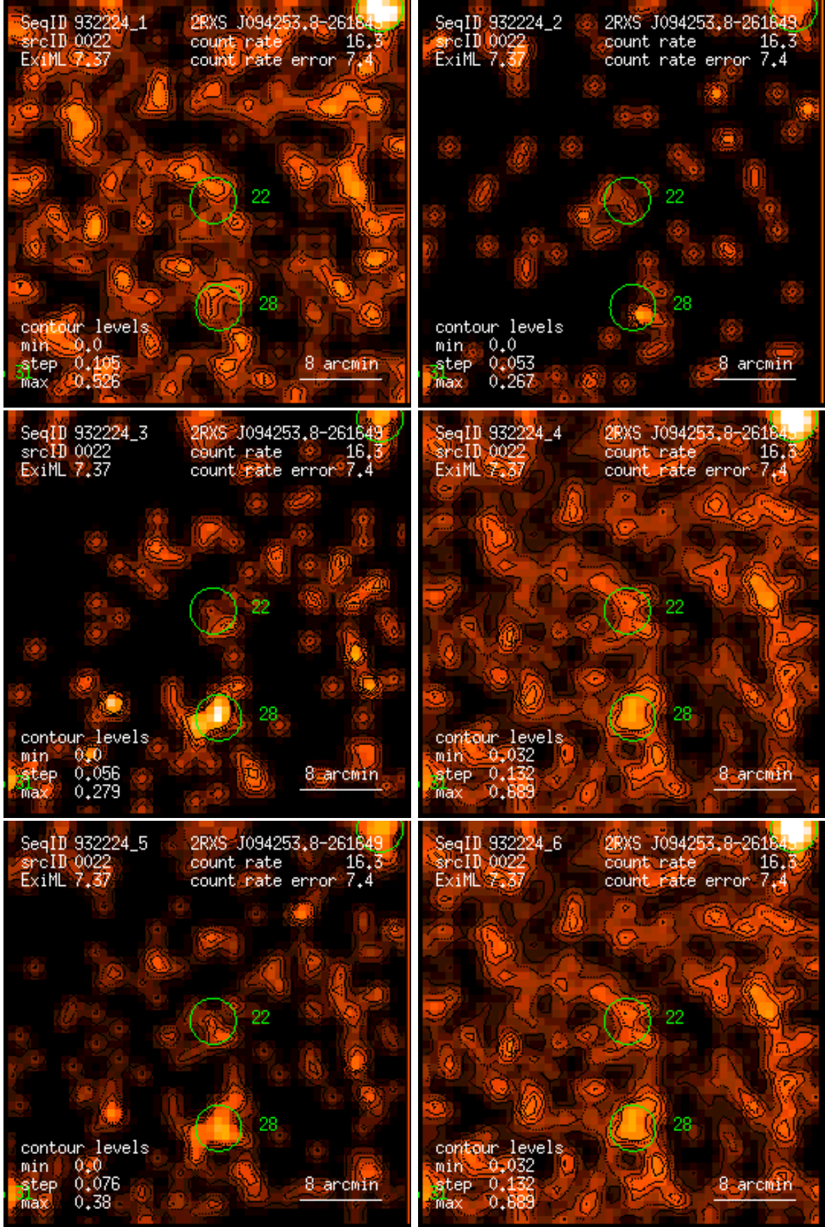
Figure 22: RASS 932224: detection 0022: band rate images, Gaussian filter: (1) PSPC channels 11 – 41, (2) 52 – 90, (3) 91 – 201, (4) 11 – 235, (5) 52 – 201, (6) 11 – 201. Broad band rates in counts/ks. Band rate contour levels in counts/ks/arcmin 2 .
