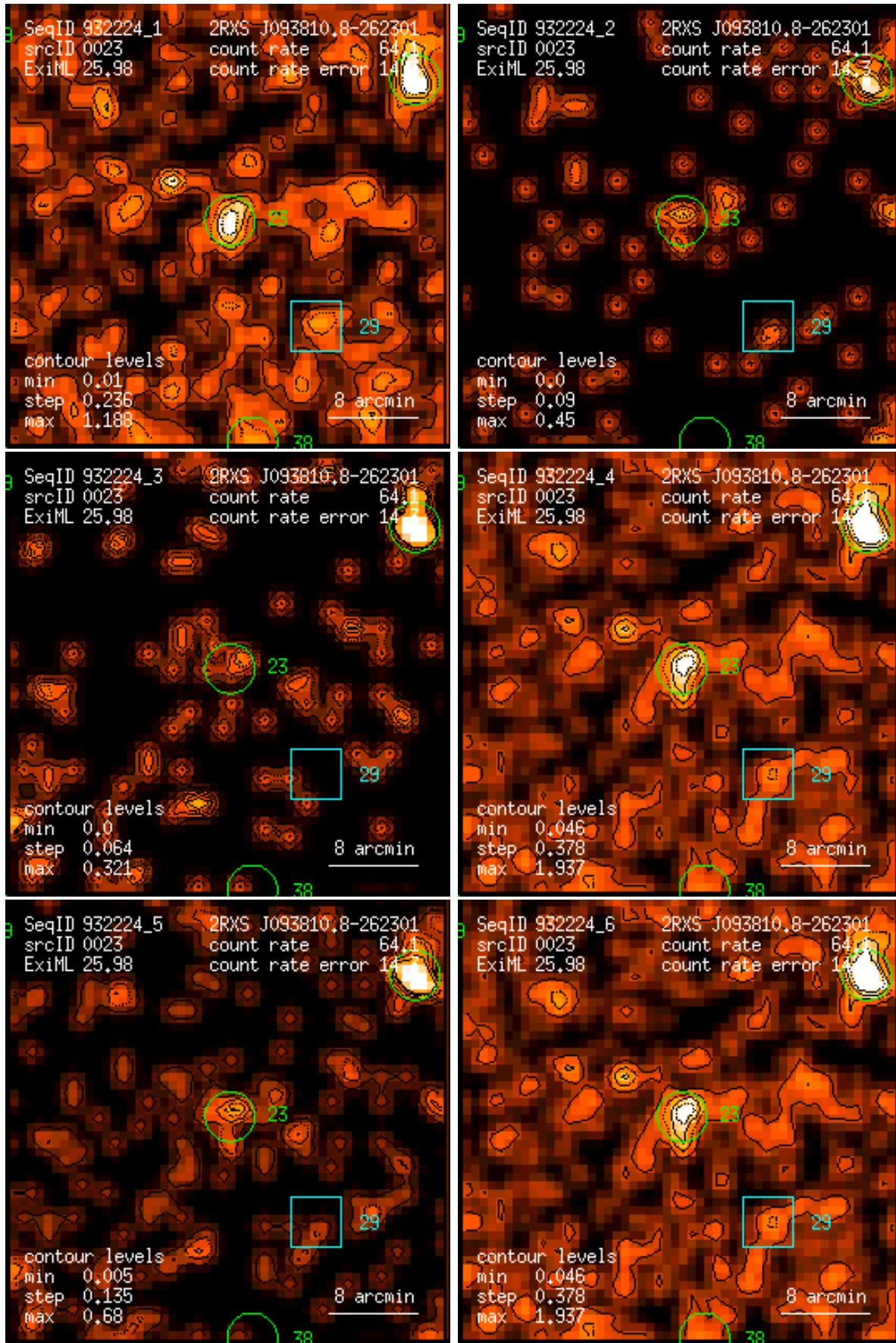
Figure 23: RASS 932224: detection 0023: band rate images, Gaussian filter: (1) PSPC channels 11 – 41, (2) 52 – 90, (3) 91 – 201, (4) 11 – 235, (5) 52 – 201, (6) 11 – 201. Broad band rates in counts/ks. Band rate contour levels in counts/ks/arcmin 2 .
