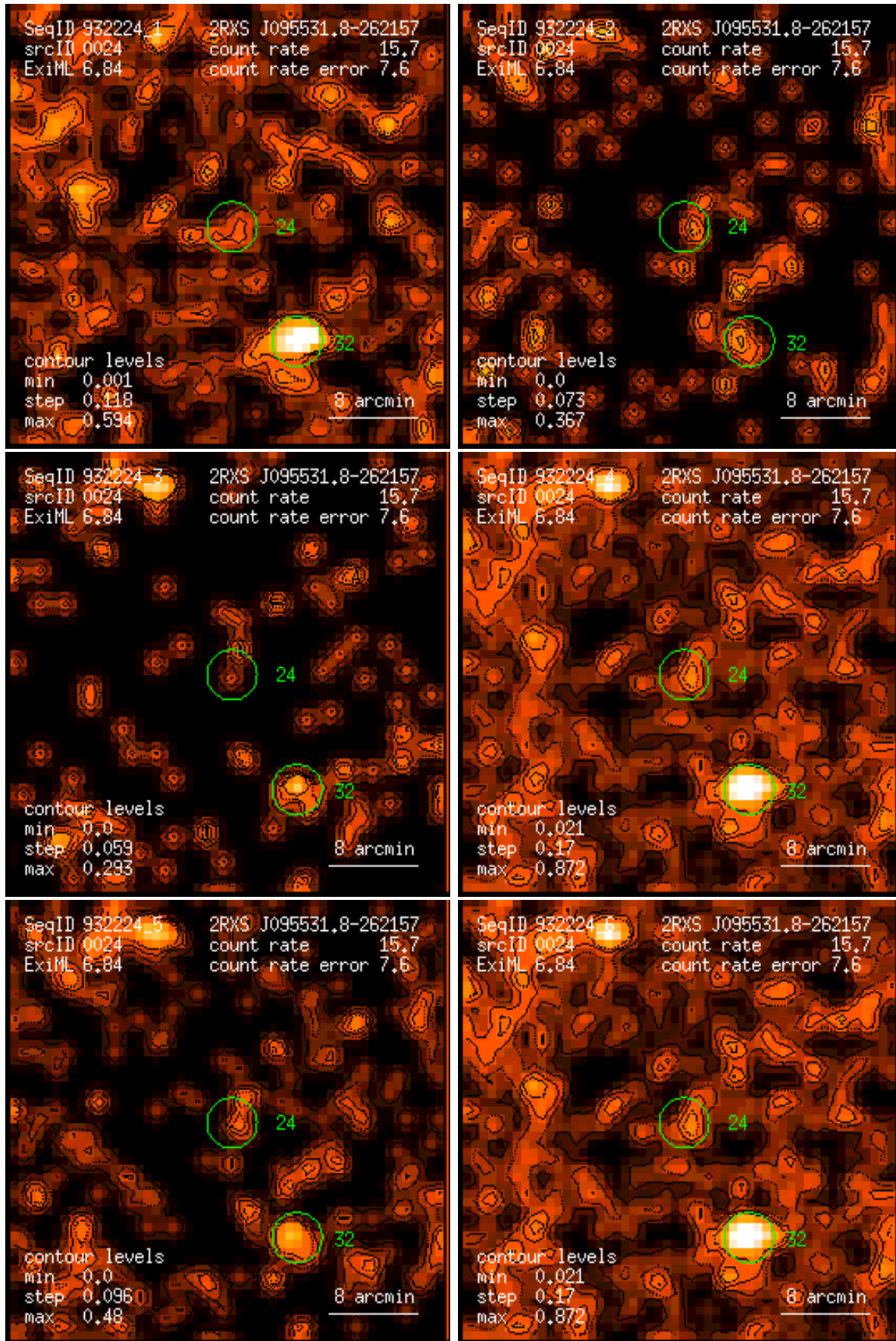
Figure 24: RASS 932224: detection 0024: band rate images, Gaussian filter: (1) PSPC channels 11 – 41, (2) 52 – 90, (3) 91 – 201, (4) 11 – 235, (5) 52 – 201, (6) 11 – 201. Broad band rates in counts/ks. Band rate contour levels in counts/ks/arcmin 2 .
