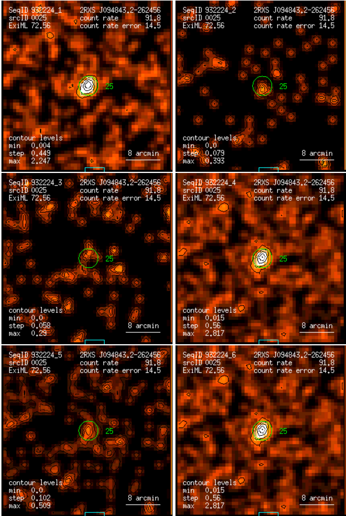
Figure 25: RASS 932224: detection 0025: band rate images, Gaussian filter: (1) PSPC channels 11 – 41, (2) 52 – 90, (3) 91 – 201, (4) 11 – 235, (5) 52 – 201, (6) 11 – 201. Broad band rates in counts/ks. Band rate contour levels in counts/ks/arcmin 2 .
