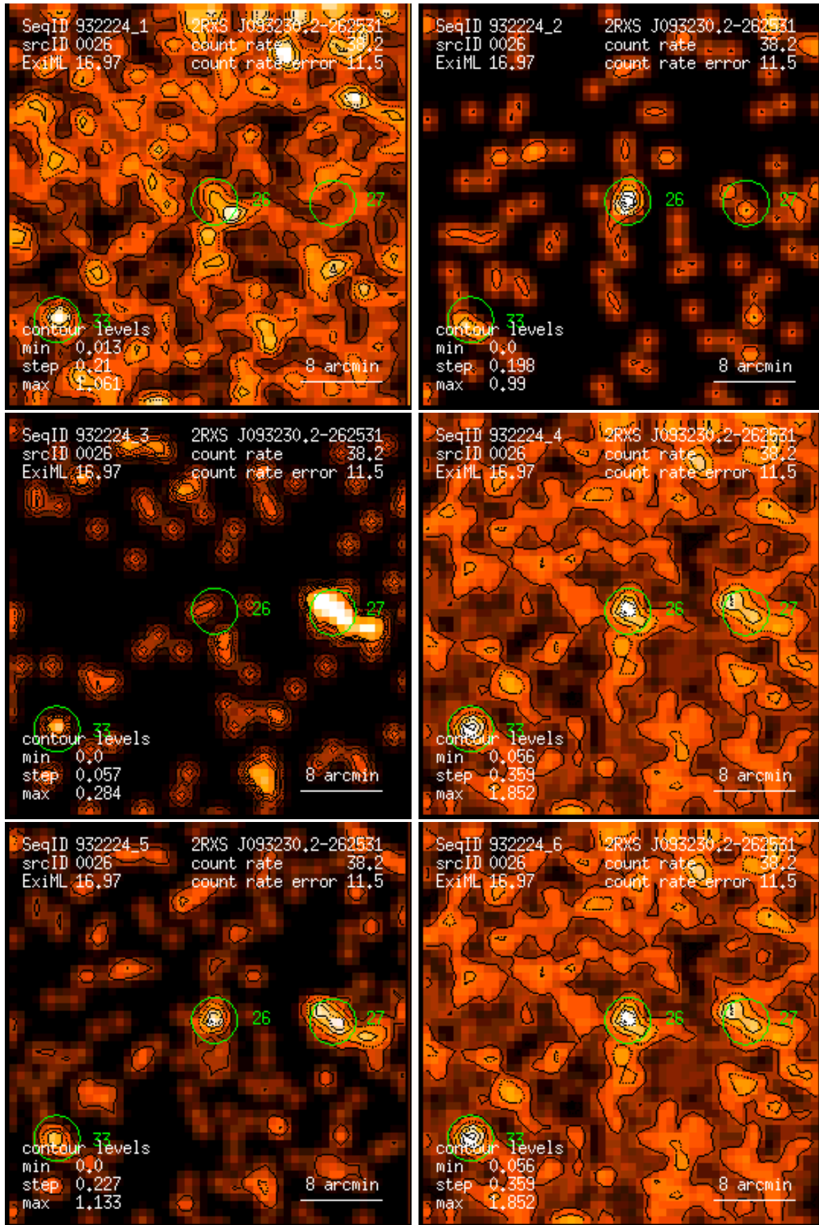
Figure 26: RASS 932224: detection 0026: band rate images, Gaussian filter: (1) PSPC channels 11 – 41, (2) 52 – 90, (3) 91 – 201, (4) 11 – 235, (5) 52 – 201, (6) 11 – 201. Broad band rates in counts/ks. Band rate contour levels in counts/ks/arcmin 2 .
