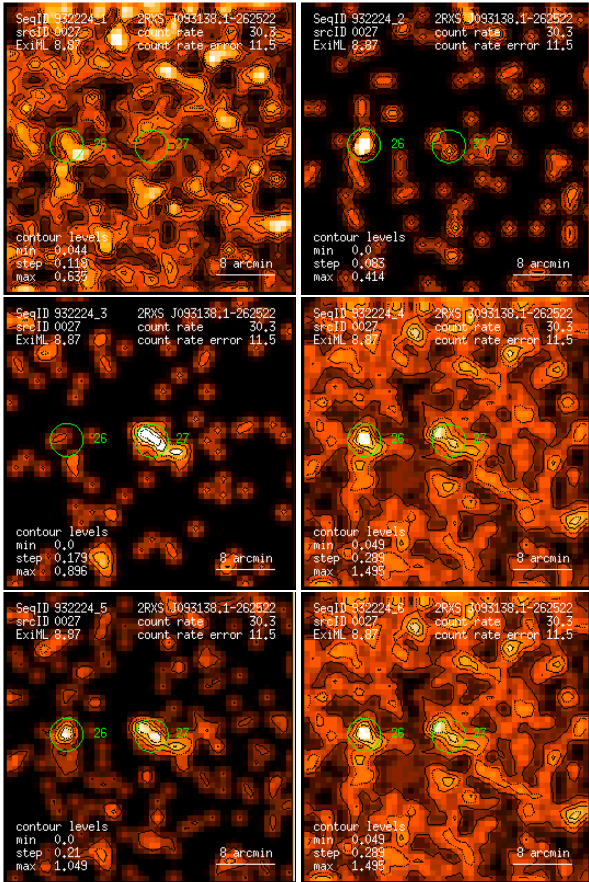
Figure 27: RASS 932224: detection 0027: band rate images, Gaussian filter: (1) PSPC channels 11 – 41, (2) 52 – 90, (3) 91 – 201, (4) 11 – 235, (5) 52 – 201, (6) 11 – 201. Broad band rates in counts/ks. Band rate contour levels in counts/ks/arcmin 2 .
