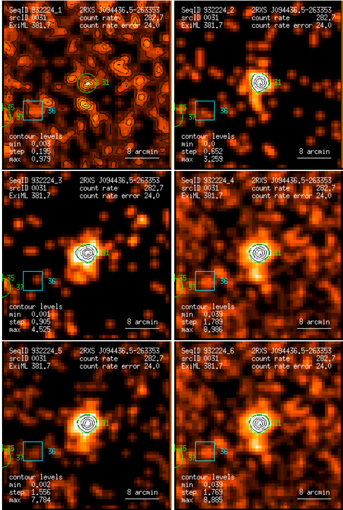
Figure 31: RASS 932224: detection 0031: band rate images, Gaussian filter: (1) PSPC channels 11 – 41, (2) 52 – 90, (3) 91 – 201, (4) 11 – 235, (5) 52 – 201, (6) 11 – 201. Broad band rates in counts/ks. Band rate contour levels in counts/ks/arcmin 2 .
