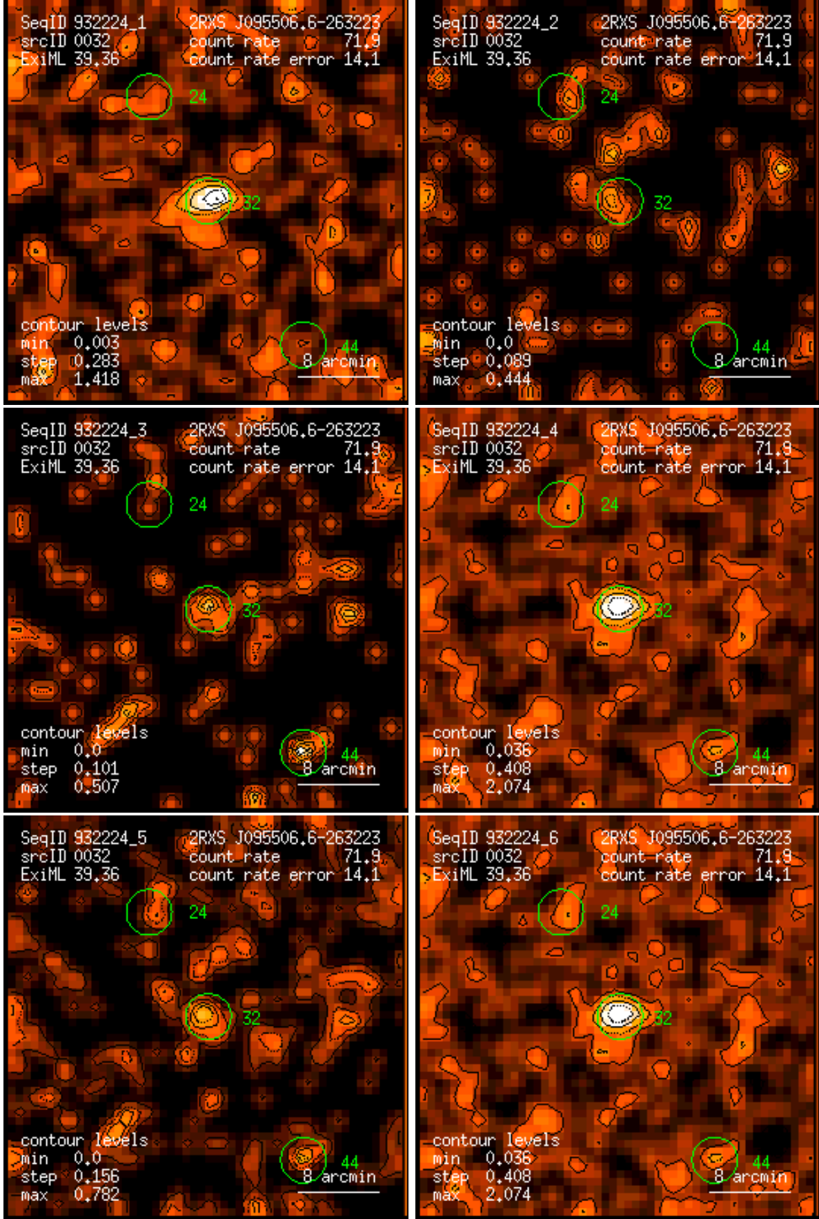
Figure 32: RASS 932224: detection 0032: band rate images, Gaussian filter: (1) PSPC channels 11 – 41, (2) 52 – 90, (3) 91 – 201, (4) 11 – 235, (5) 52 – 201, (6) 11 – 201. Broad band rates in counts/ks. Band rate contour levels in counts/ks/arcmin 2 .
