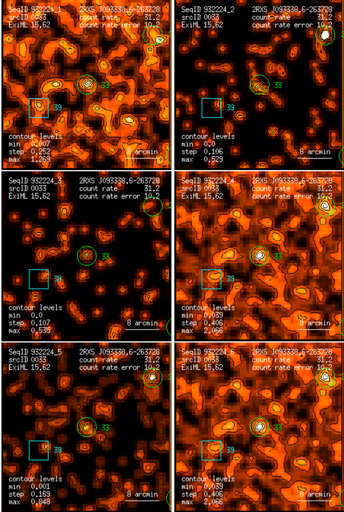
Figure 33: RASS 932224: detection 0033: band rate images, Gaussian filter: (1) PSPC channels 11 – 41, (2) 52 – 90, (3) 91 – 201, (4) 11 – 235, (5) 52 – 201, (6) 11 – 201. Broad band rates in counts/ks. Band rate contour levels in counts/ks/arcmin 2 .
