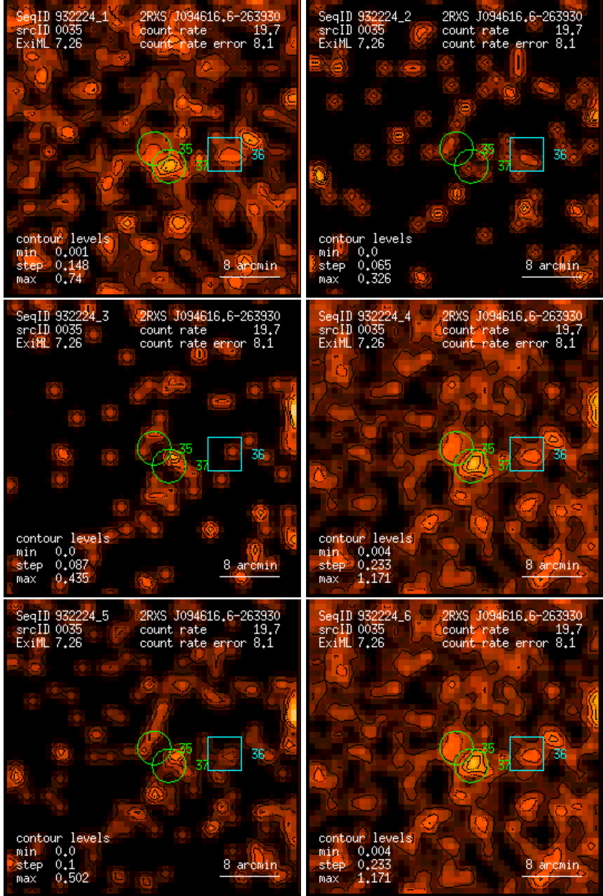
Figure 35: RASS 932224: detection 0035: band rate images, Gaussian filter: (1) PSPC channels 11 – 41, (2) 52 – 90, (3) 91 – 201, (4) 11 – 235, (5) 52 – 201, (6) 11 – 201. Broad band rates in counts/ks. Band rate contour levels in counts/ks/arcmin 2 .
