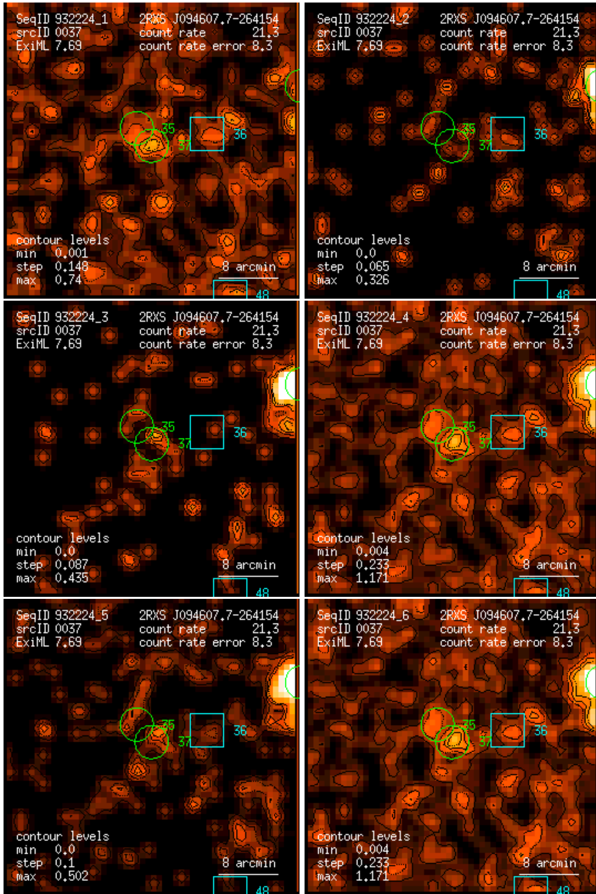
Figure 37: RASS 932224: detection 0037: band rate images, Gaussian filter: (1) PSPC channels 11 – 41, (2) 52 – 90, (3) 91 – 201, (4) 11 – 235, (5) 52 – 201, (6) 11 – 201. Broad band rates in counts/ks. Band rate contour levels in counts/ks/arcmin 2 .
