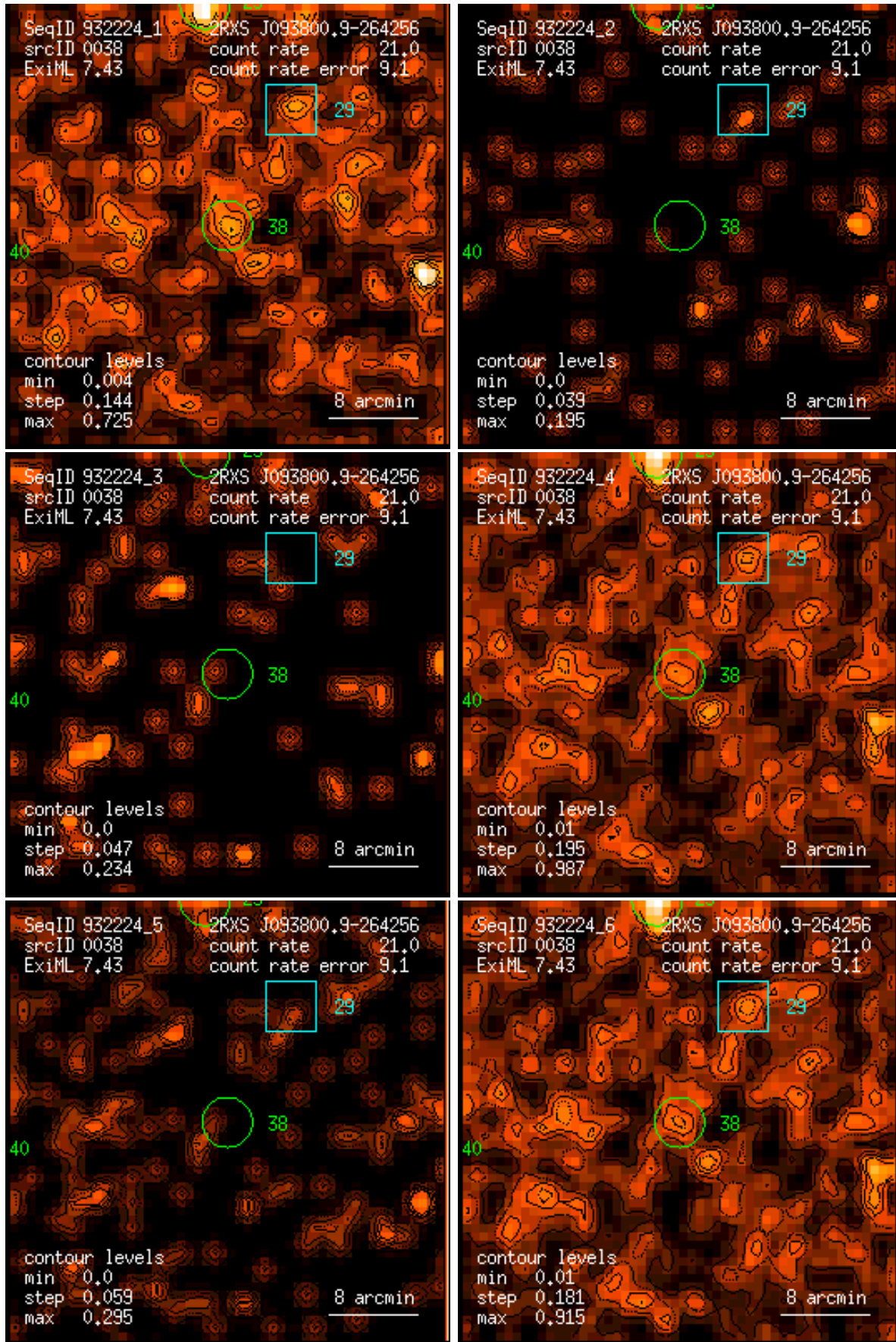
Figure 38: RASS 932224: detection 0038: band rate images, Gaussian filter: (1) PSPC channels 11 – 41, (2) 52 – 90, (3) 91 – 201, (4) 11 – 235, (5) 52 – 201, (6) 11 – 201. Broad band rates in counts/ks. Band rate contour levels in counts/ks/arcmin 2 .
