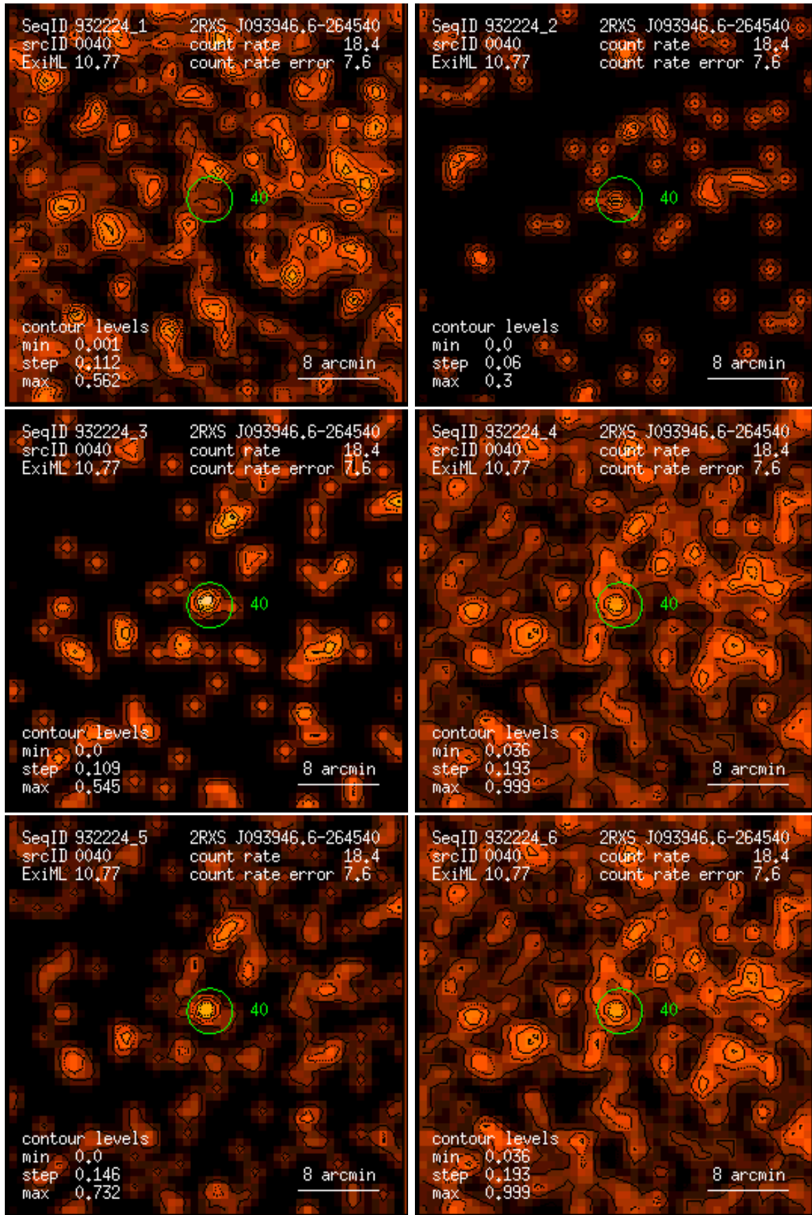
Figure 40: RASS 932224: detection 0040: band rate images, Gaussian filter: (1) PSPC channels 11 – 41, (2) 52 – 90, (3) 91 – 201, (4) 11 – 235, (5) 52 – 201, (6) 11 – 201. Broad band rates in counts/ks. Band rate contour levels in counts/ks/arcmin 2 .
