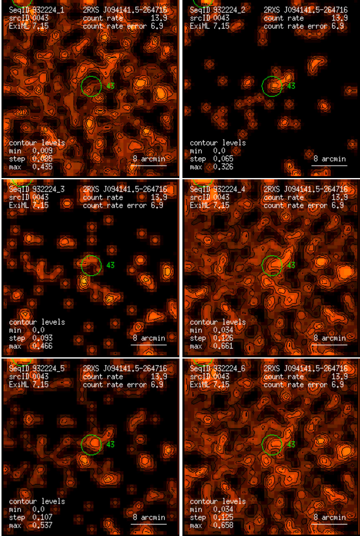
Figure 43: RASS 932224: detection 0043: band rate images, Gaussian filter: (1) PSPC channels 11 – 41, (2) 52 – 90, (3) 91 – 201, (4) 11 – 235, (5) 52 – 201, (6) 11 – 201. Broad band rates in counts/ks. Band rate contour levels in counts/ks/arcmin 2 .
