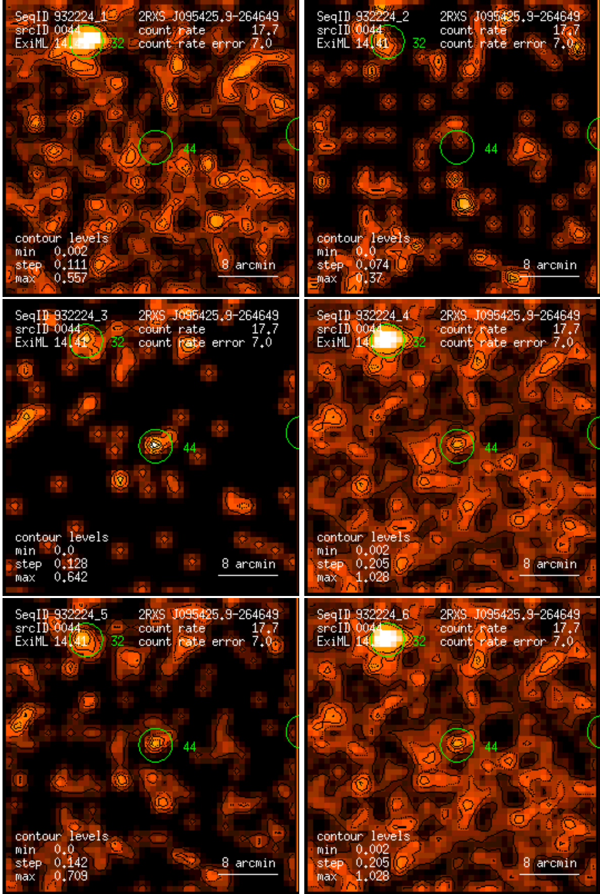
Figure 44: RASS 932224: detection 0044: band rate images, Gaussian filter: (1) PSPC channels 11 – 41, (2) 52 – 90, (3) 91 – 201, (4) 11 – 235, (5) 52 – 201, (6) 11 – 201. Broad band rates in counts/ks. Band rate contour levels in counts/ks/arcmin 2 .
