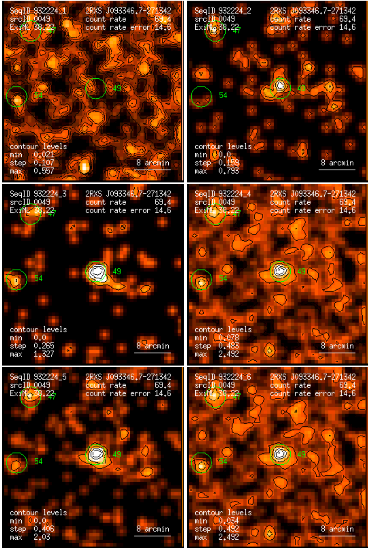
Figure 49: RASS 932224: detection 0049: band rate images, Gaussian filter: (1) PSPC channels 11 – 41, (2) 52 – 90, (3) 91 – 201, (4) 11 – 235, (5) 52 – 201, (6) 11 – 201. Broad band rates in counts/ks. Band rate contour levels in counts/ks/arcmin 2 .
