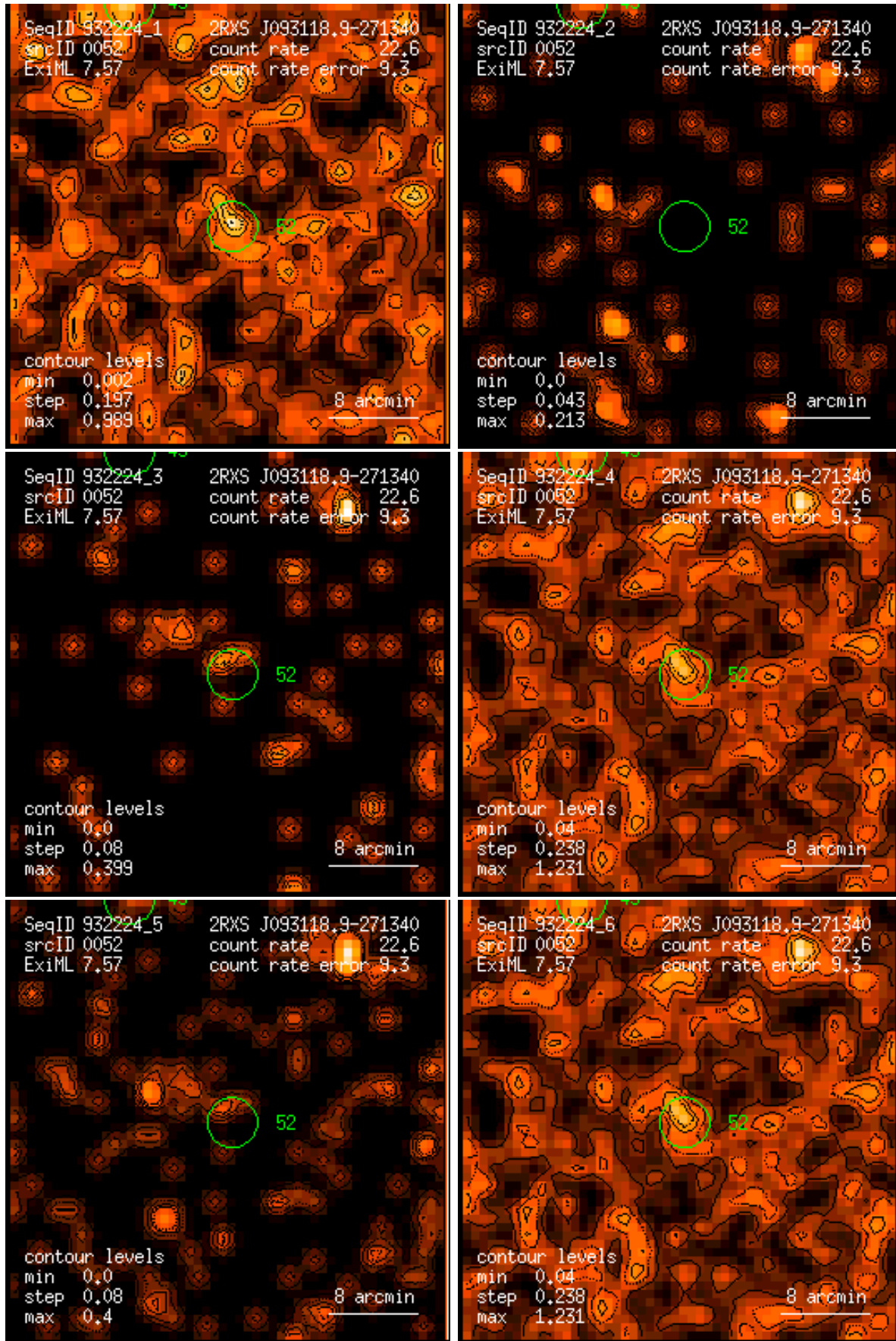
Figure 52: RASS 932224: detection 0052: band rate images, Gaussian filter: (1) PSPC channels 11 – 41, (2) 52 – 90, (3) 91 – 201, (4) 11 – 235, (5) 52 – 201, (6) 11 – 201. Broad band rates in counts/ks. Band rate contour levels in counts/ks/arcmin 2 .
