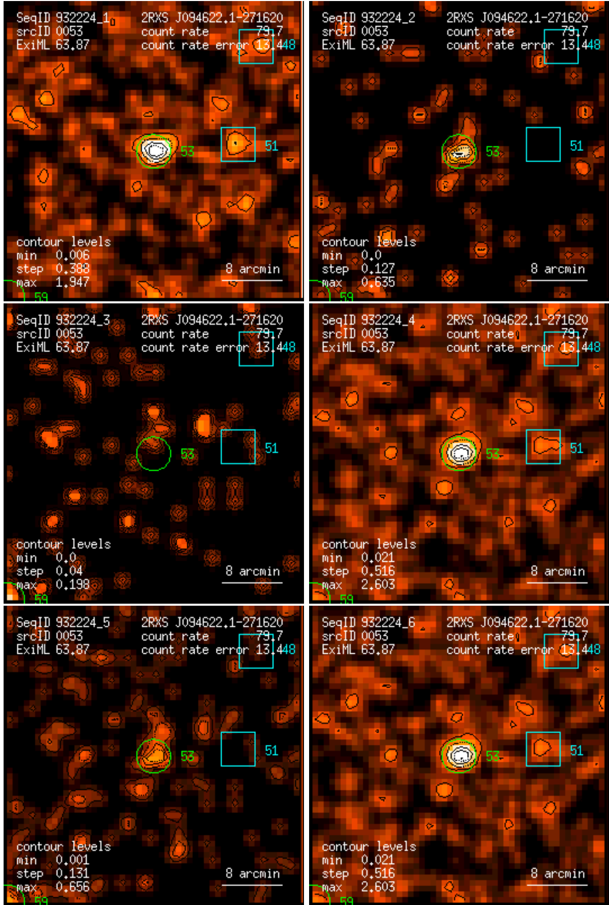
Figure 53: RASS 932224: detection 0053: band rate images, Gaussian filter: (1) PSPC channels 11 – 41, (2) 52 – 90, (3) 91 – 201, (4) 11 – 235, (5) 52 – 201, (6) 11 – 201. Broad band rates in counts/ks. Band rate contour levels in counts/ks/arcmin 2 .
