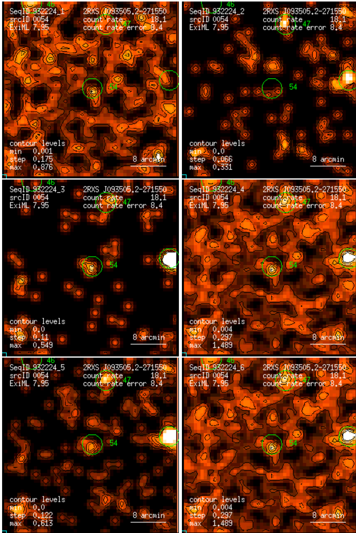
Figure 54: RASS 932224: detection 0054: band rate images, Gaussian filter: (1) PSPC channels 11 – 41, (2) 52 – 90, (3) 91 – 201, (4) 11 – 235, (5) 52 – 201, (6) 11 – 201. Broad band rates in counts/ks. Band rate contour levels in counts/ks/arcmin 2 .
