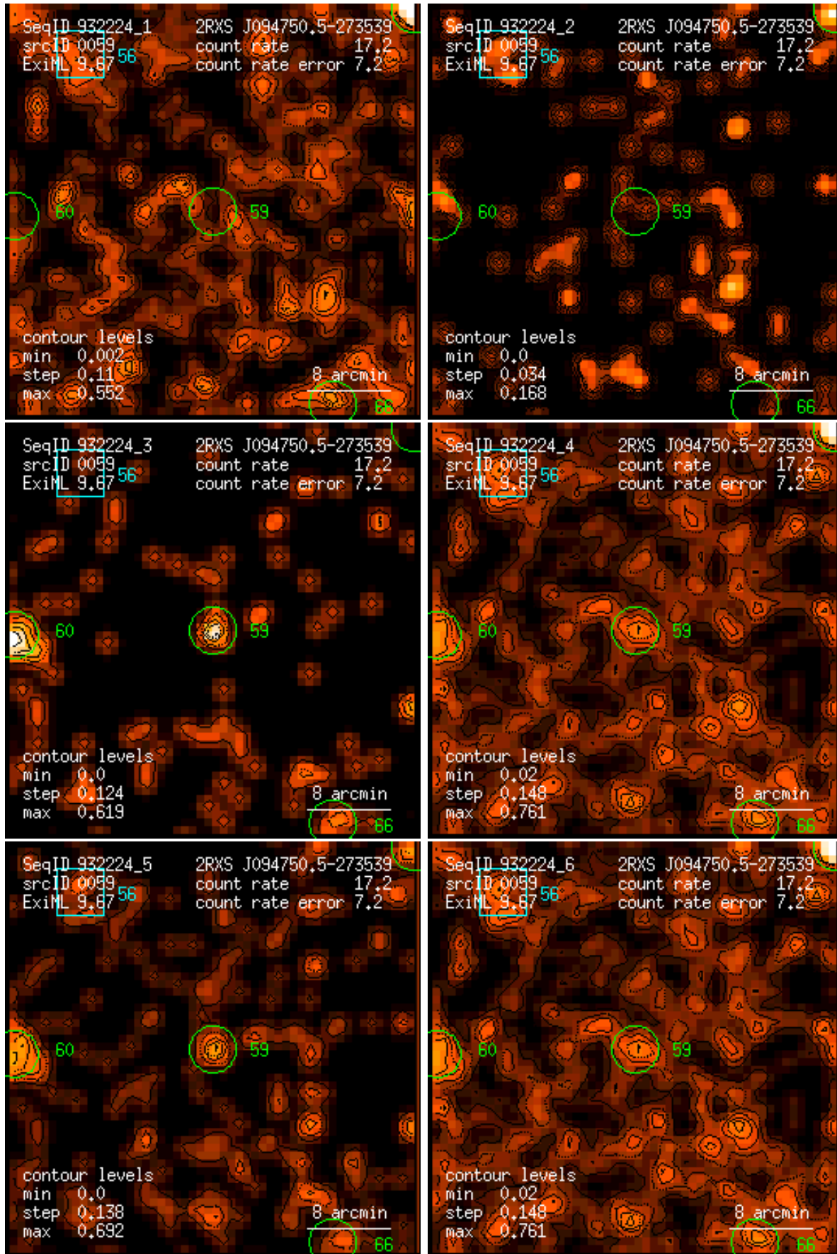
Figure 59: RASS 932224: detection 0059: band rate images, Gaussian filter: (1) PSPC channels 11 – 41, (2) 52 – 90, (3) 91 – 201, (4) 11 – 235, (5) 52 – 201, (6) 11 – 201. Broad band rates in counts/ks. Band rate contour levels in counts/ks/arcmin 2 .
