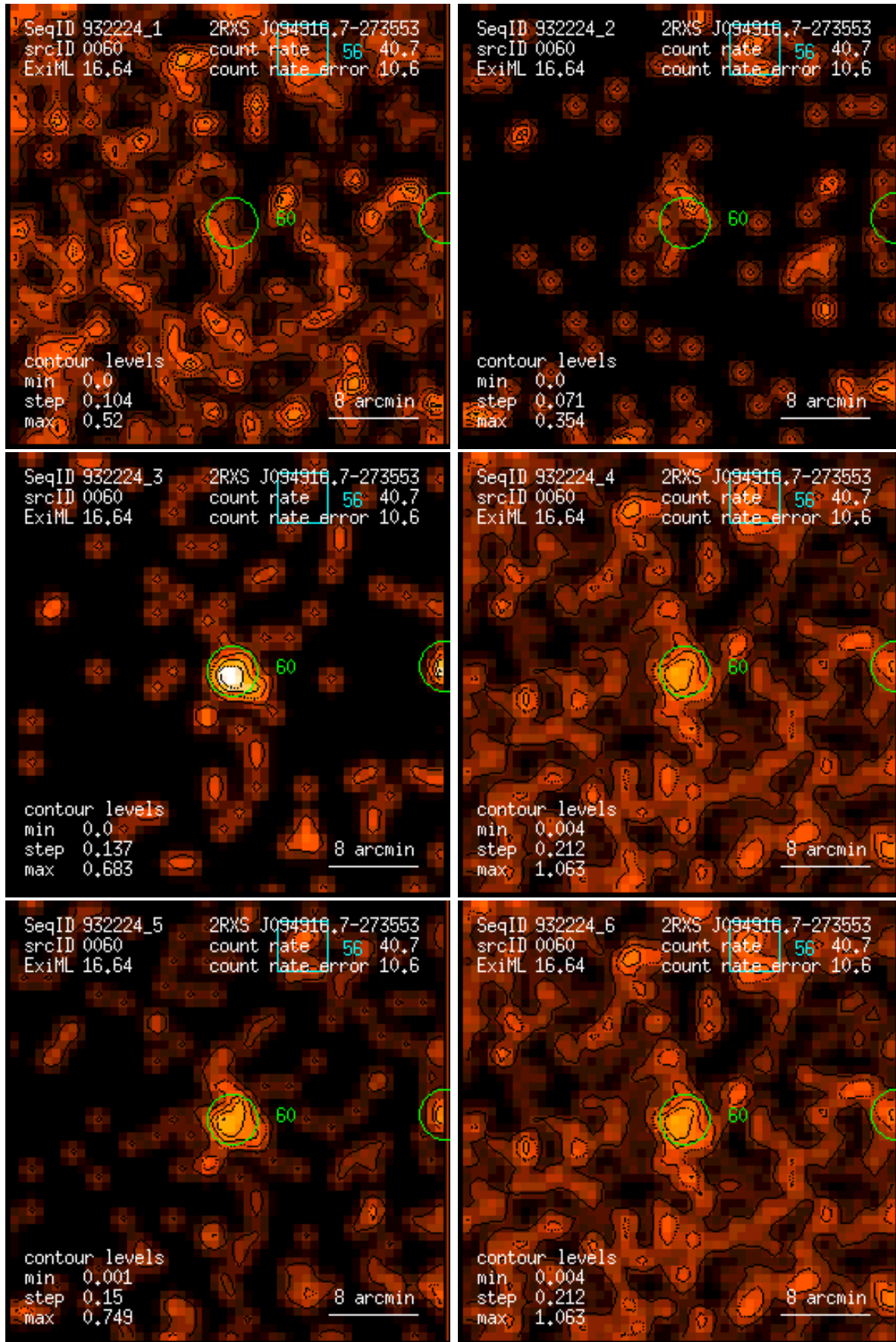
Figure 60: RASS 932224: detection 0060: band rate images, Gaussian filter: (1) PSPC channels 11 – 41, (2) 52 – 90, (3) 91 – 201, (4) 11 – 235, (5) 52 – 201, (6) 11 – 201. Broad band rates in counts/ks. Band rate contour levels in counts/ks/arcmin 2 .
