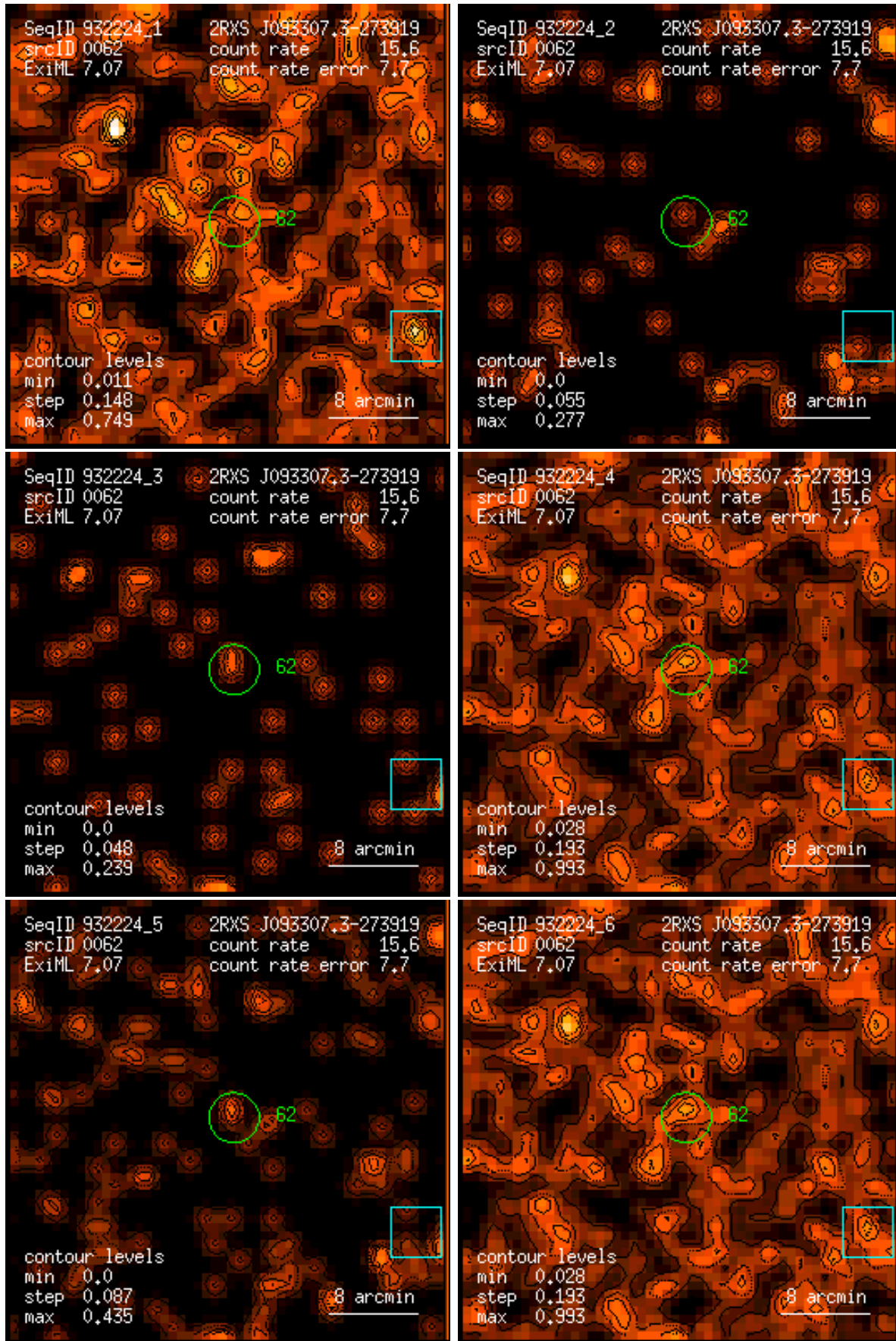
Figure 62: RASS 932224: detection 0062: band rate images, Gaussian filter: (1) PSPC channels 11 – 41, (2) 52 – 90, (3) 91 – 201, (4) 11 – 235, (5) 52 – 201, (6) 11 – 201. Broad band rates in counts/ks. Band rate contour levels in counts/ks/arcmin 2 .
