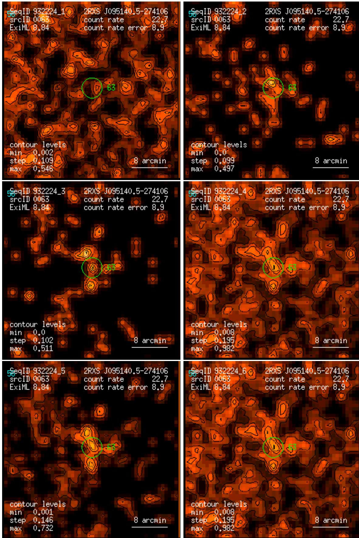
Figure 63: RASS 932224: detection 0063: band rate images, Gaussian filter: (1) PSPC channels 11 – 41, (2) 52 – 90, (3) 91 – 201, (4) 11 – 235, (5) 52 – 201, (6) 11 – 201. Broad band rates in counts/ks. Band rate contour levels in counts/ks/arcmin 2 .
