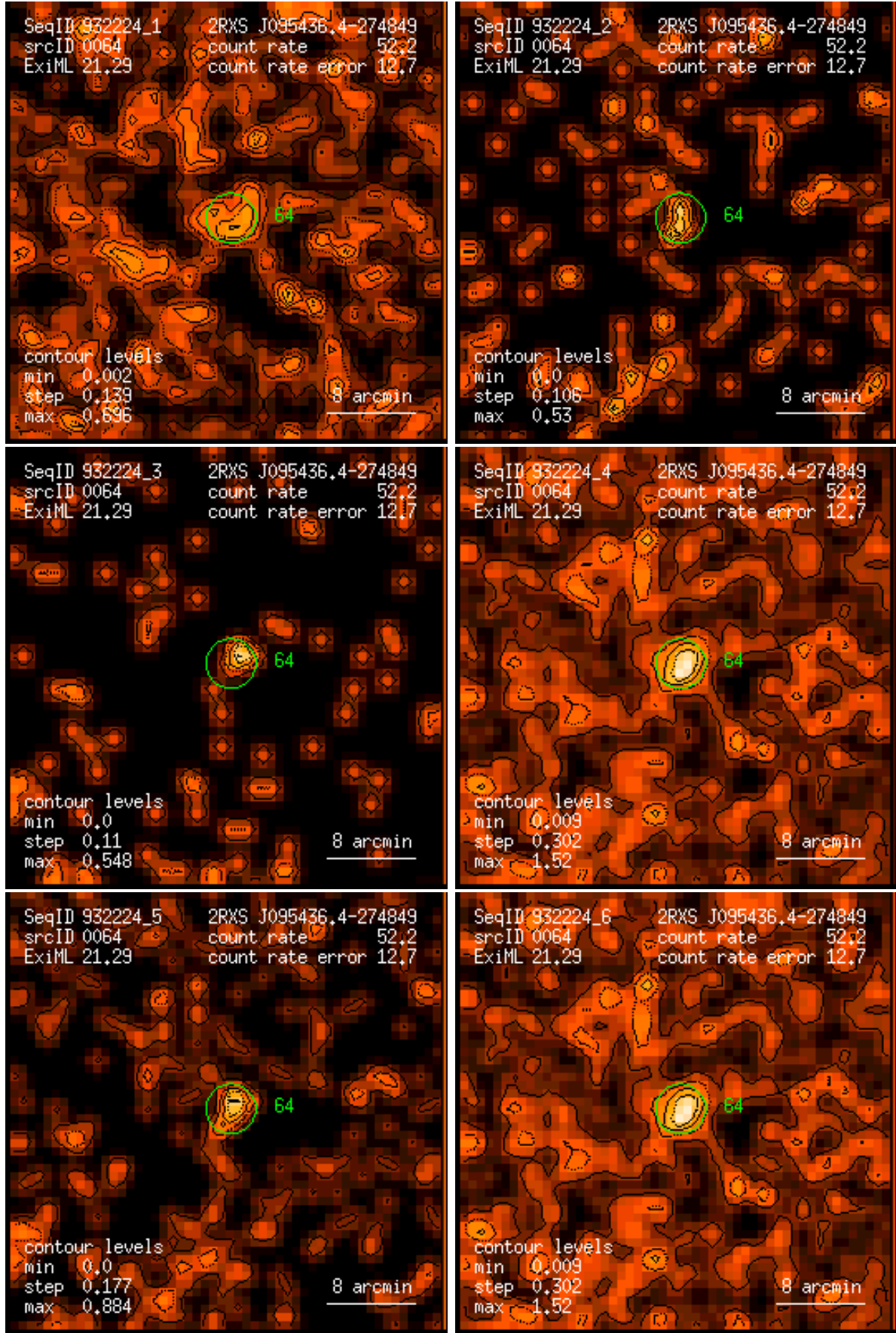
Figure 64: RASS 932224: detection 0064: band rate images, Gaussian filter: (1) PSPC channels 11 – 41, (2) 52 – 90, (3) 91 – 201, (4) 11 – 235, (5) 52 – 201, (6) 11 – 201. Broad band rates in counts/ks. Band rate contour levels in counts/ks/arcmin 2 .
