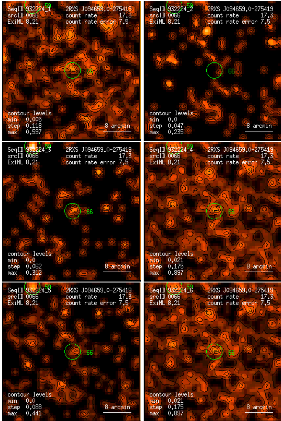
Figure 66: RASS 932224: detection 0066: band rate images, Gaussian filter: (1) PSPC channels 11 – 41, (2) 52 – 90, (3) 91 – 201, (4) 11 – 235, (5) 52 – 201, (6) 11 – 201. Broad band rates in counts/ks. Band rate contour levels in counts/ks/arcmin 2 .
