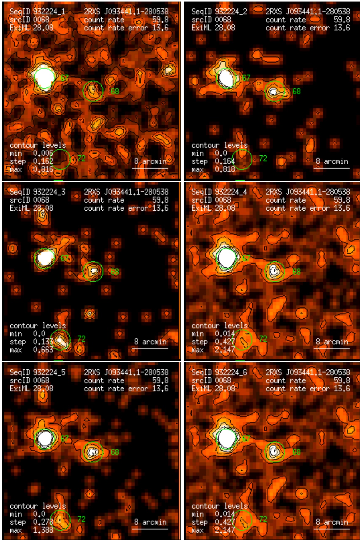
Figure 68: RASS 932224: detection 0068: band rate images, Gaussian filter: (1) PSPC channels 11 – 41, (2) 52 – 90, (3) 91 – 201, (4) 11 – 235, (5) 52 – 201, (6) 11 – 201. Broad band rates in counts/ks. Band rate contour levels in counts/ks/arcmin 2 .
