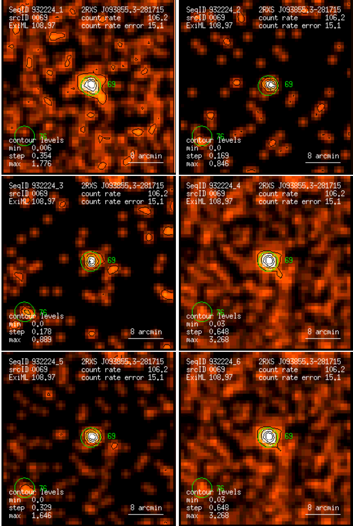
Figure 69: RASS 932224: detection 0069: band rate images, Gaussian filter: (1) PSPC channels 11 – 41, (2) 52 – 90, (3) 91 – 201, (4) 11 – 235, (5) 52 – 201, (6) 11 – 201. Broad band rates in counts/ks. Band rate contour levels in counts/ks/arcmin 2 .
