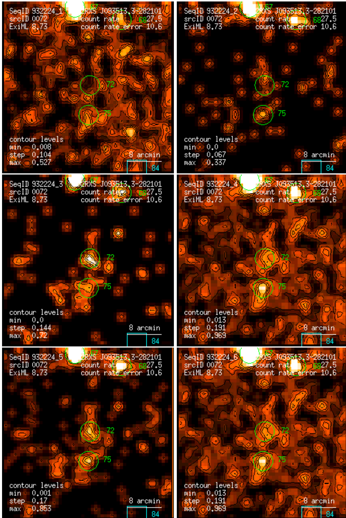
Figure 72: RASS 932224: detection 0072: band rate images, Gaussian filter: (1) PSPC channels 11 – 41, (2) 52 – 90, (3) 91 – 201, (4) 11 – 235, (5) 52 – 201, (6) 11 – 201. Broad band rates in counts/ks. Band rate contour levels in counts/ks/arcmin 2 .
