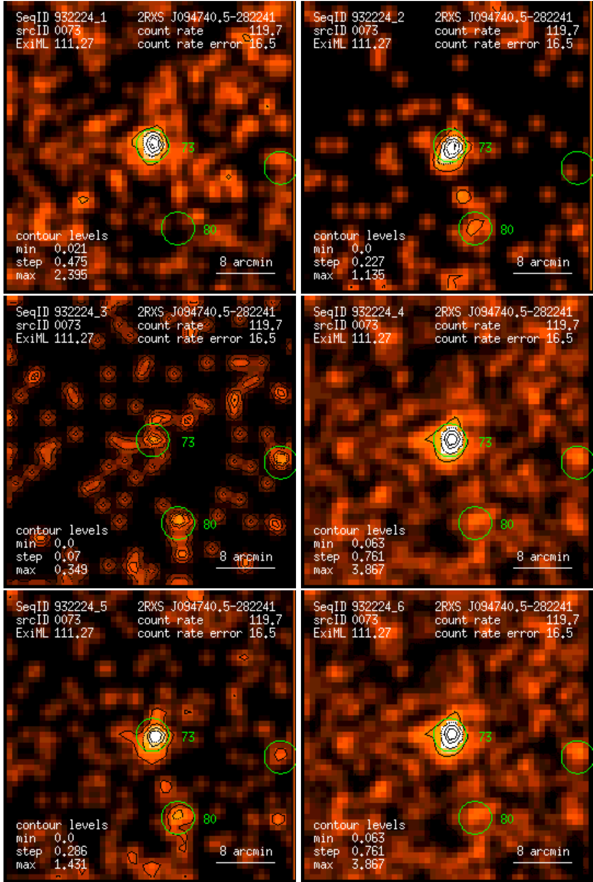
Figure 73: RASS 932224: detection 0073: band rate images, Gaussian filter: (1) PSPC channels 11 – 41, (2) 52 – 90, (3) 91 – 201, (4) 11 – 235, (5) 52 – 201, (6) 11 – 201. Broad band rates in counts/ks. Band rate contour levels in counts/ks/arcmin 2 .
