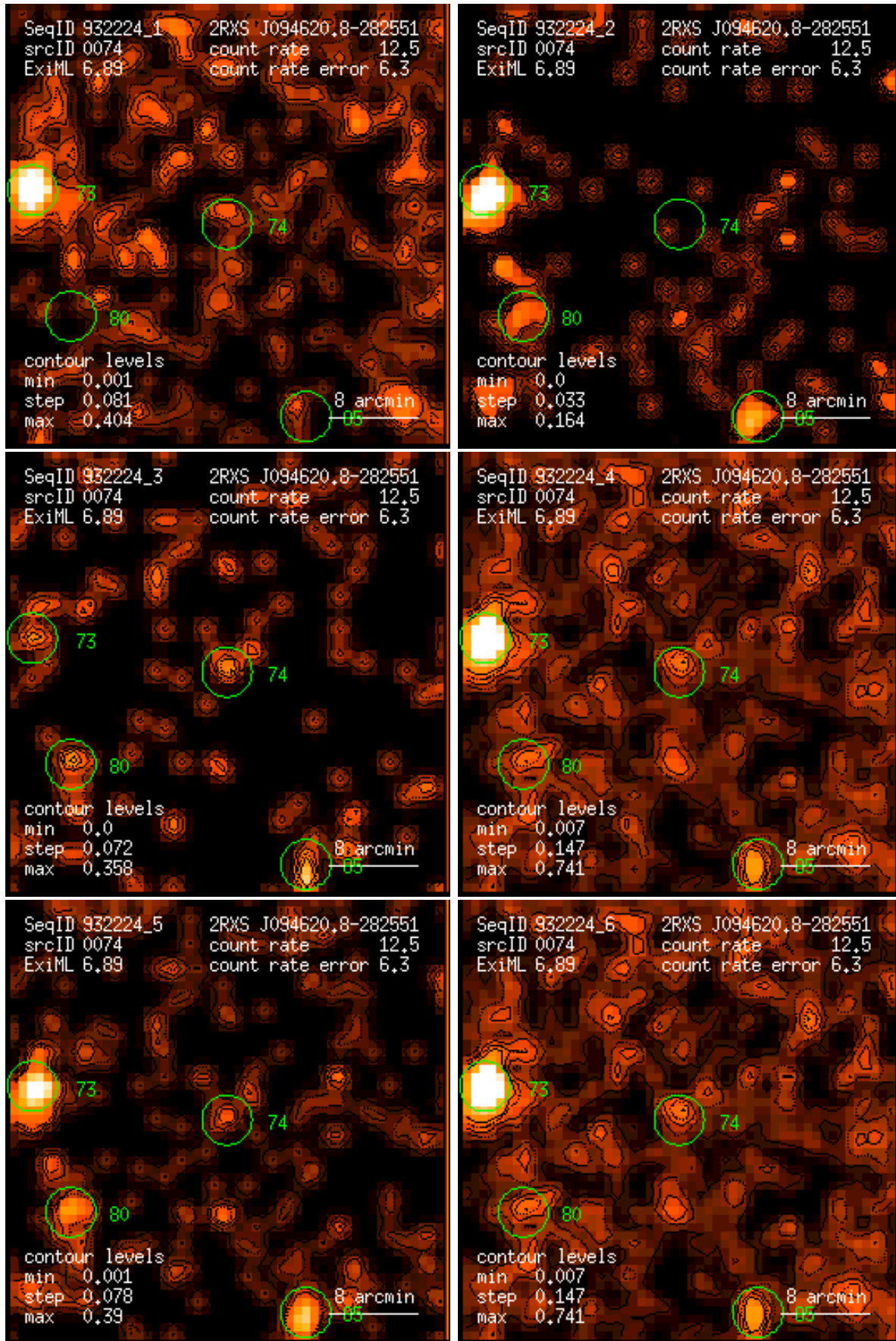
Figure 74: RASS 932224: detection 0074: band rate images, Gaussian filter: (1) PSPC channels 11 – 41, (2) 52 – 90, (3) 91 – 201, (4) 11 – 235, (5) 52 – 201, (6) 11 – 201. Broad band rates in counts/ks. Band rate contour levels in counts/ks/arcmin 2 .
