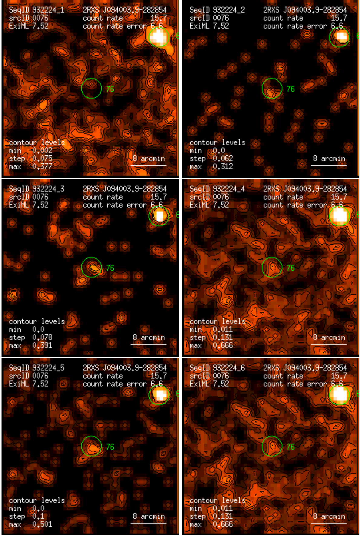
Figure 76: RASS 932224: detection 0076: band rate images, Gaussian filter: (1) PSPC channels 11 – 41, (2) 52 – 90, (3) 91 – 201, (4) 11 – 235, (5) 52 – 201, (6) 11 – 201. Broad band rates in counts/ks. Band rate contour levels in counts/ks/arcmin 2 .
