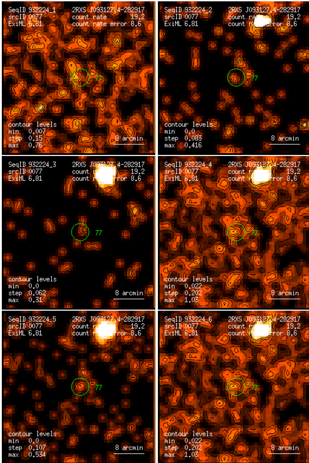
Figure 77: RASS 932224: detection 0077: band rate images, Gaussian filter: (1) PSPC channels 11 – 41, (2) 52 – 90, (3) 91 – 201, (4) 11 – 235, (5) 52 – 201, (6) 11 – 201. Broad band rates in counts/ks. Band rate contour levels in counts/ks/arcmin 2 .
