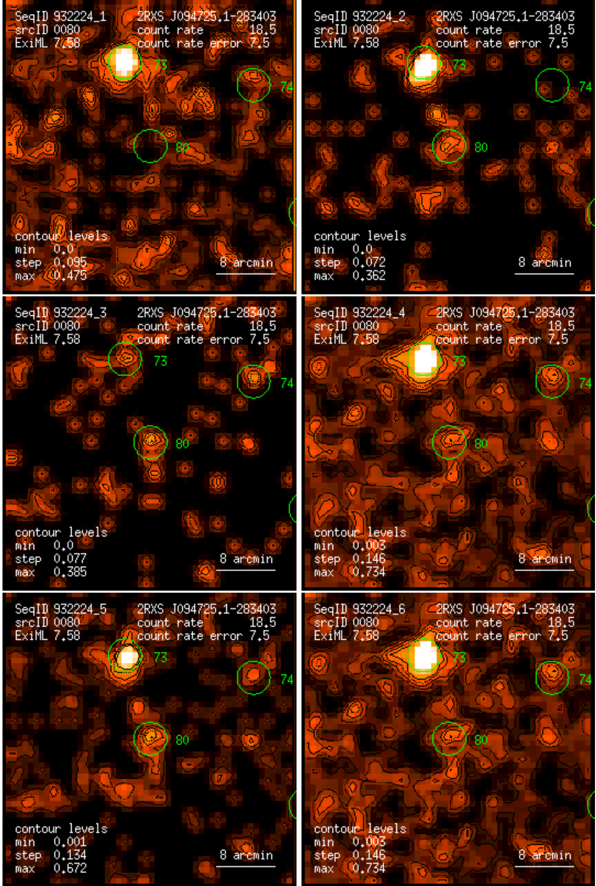
Figure 80: RASS 932224: detection 0080: band rate images, Gaussian filter: (1) PSPC channels 11 – 41, (2) 52 – 90, (3) 91 – 201, (4) 11 – 235, (5) 52 – 201, (6) 11 – 201. Broad band rates in counts/ks. Band rate contour levels in counts/ks/arcmin 2 .
