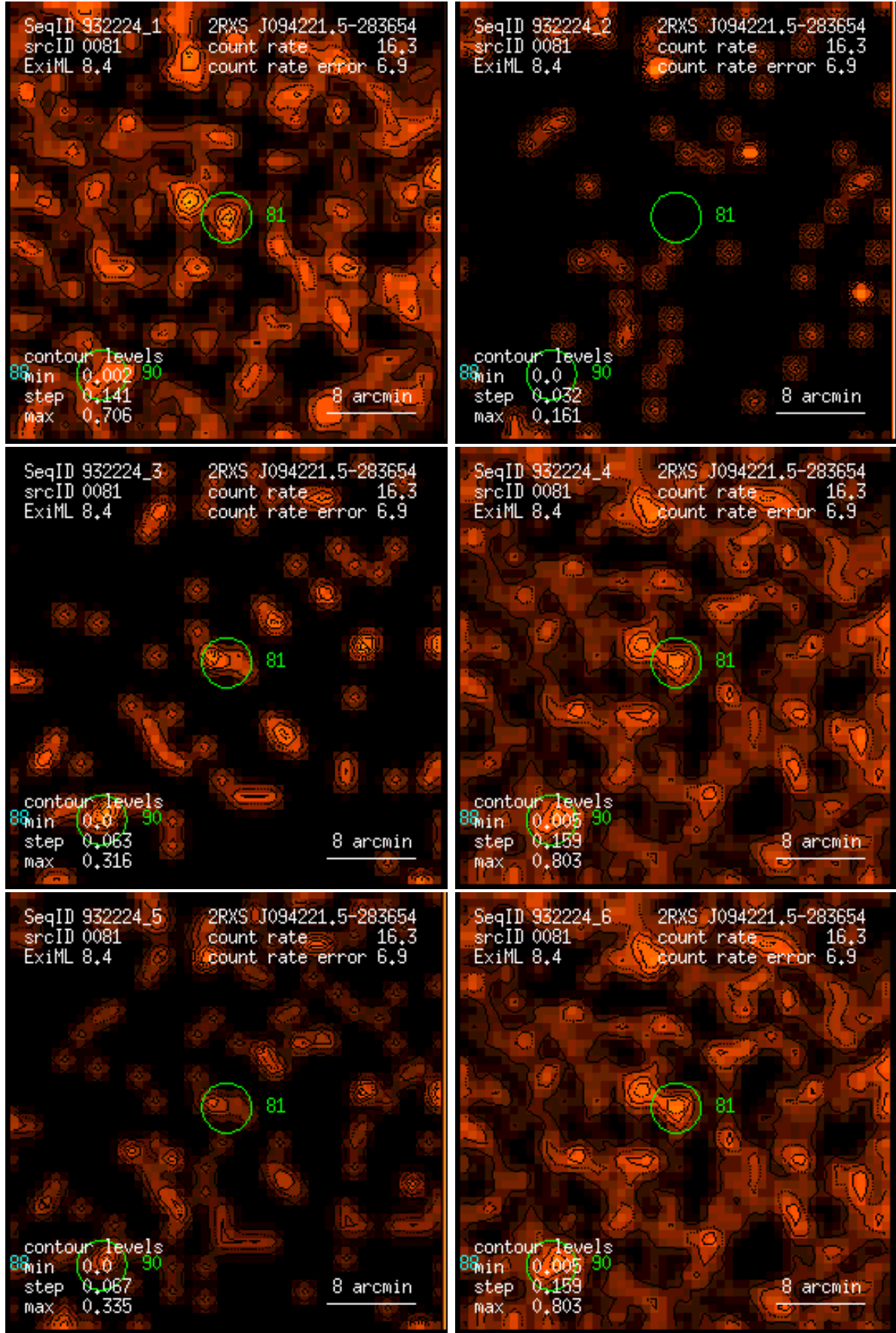
Figure 81: RASS 932224: detection 0081: band rate images, Gaussian filter: (1) PSPC channels 11 – 41, (2) 52 – 90, (3) 91 – 201, (4) 11 – 235, (5) 52 – 201, (6) 11 – 201. Broad band rates in counts/ks. Band rate contour levels in counts/ks/arcmin 2 .
