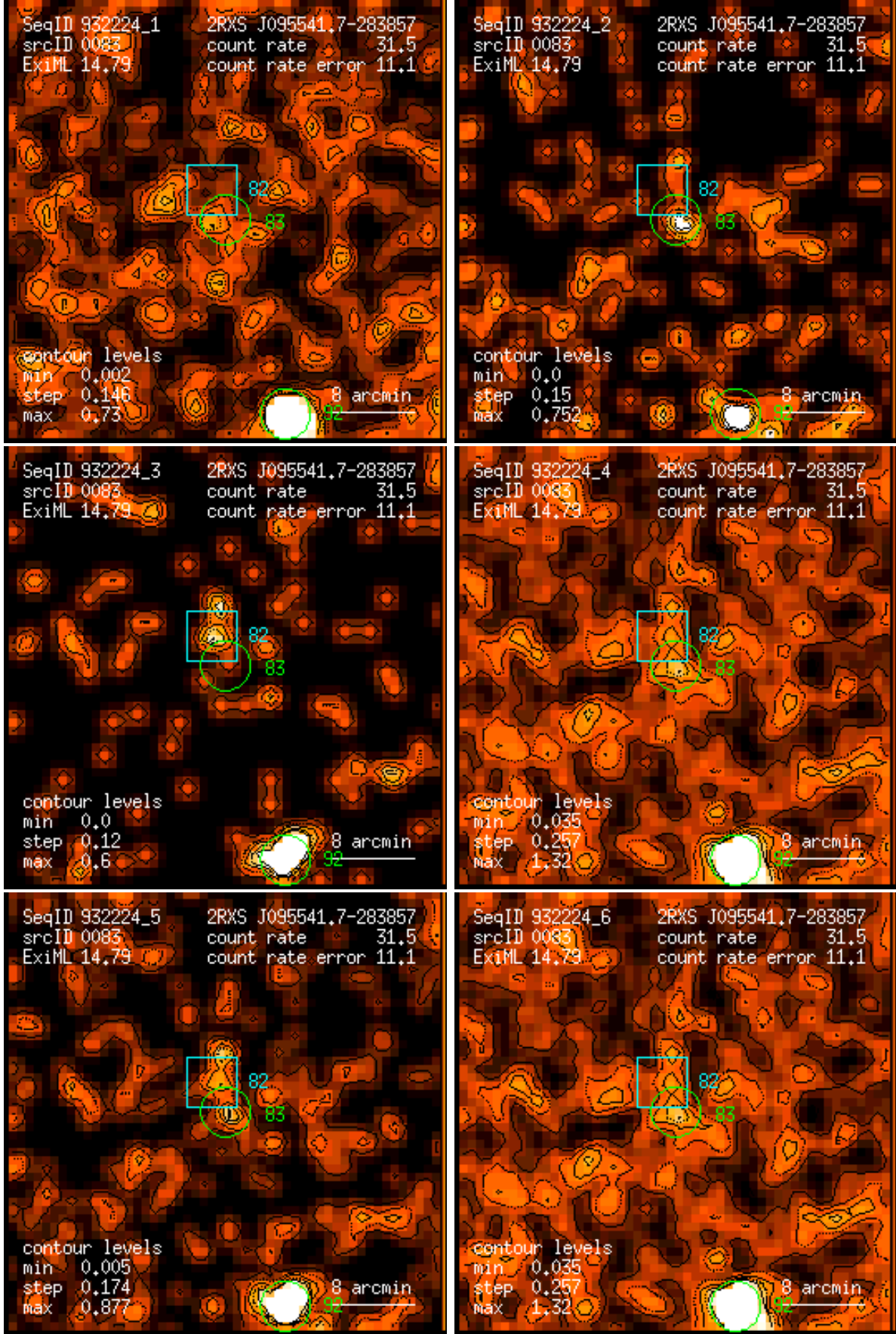
Figure 83: RASS 932224: detection 0083: band rate images, Gaussian filter: (1) PSPC channels 11 – 41, (2) 52 – 90, (3) 91 – 201, (4) 11 – 235, (5) 52 – 201, (6) 11 – 201. Broad band rates in counts/ks. Band rate contour levels in counts/ks/arcmin 2 .
